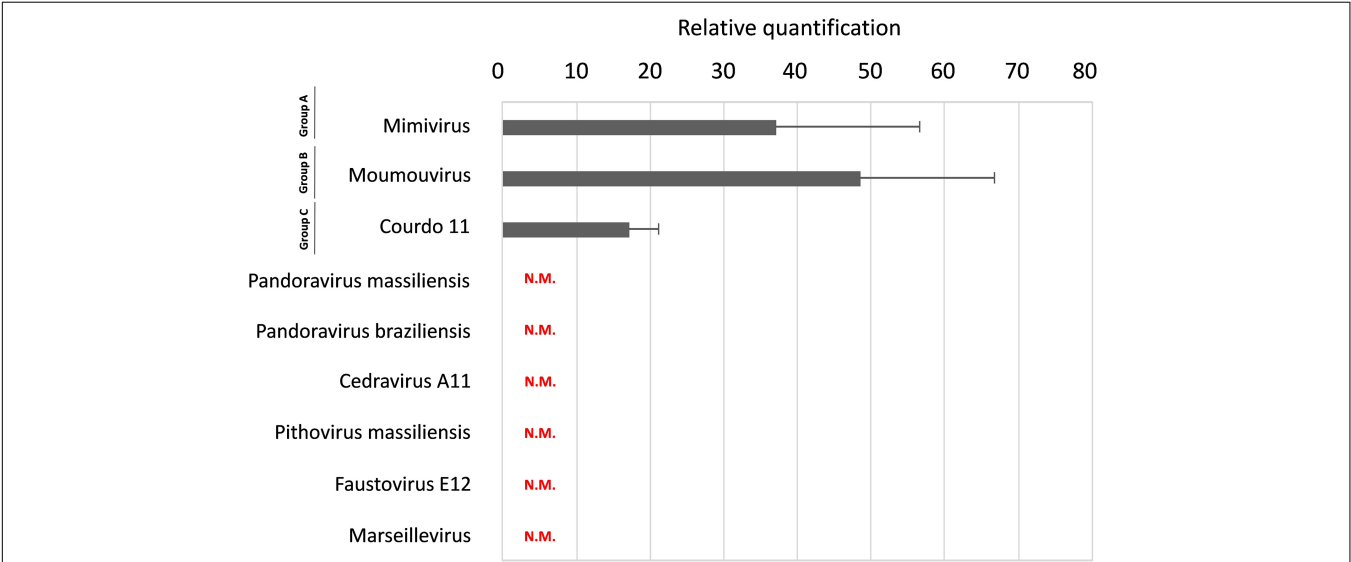
FIGURE 4 | Guarani replication in different giant viruses. Histogram of Guarani replication in different mimiviruses belonging to group A, B, C, and other giant viruses from the putative order Megavirales. The replication was calculated by the difference in the Cycle threshold (Ct) between time points H0 and H24 measured by Real-Time PCR. The results were then analyzed with the Delta Ct method. N.M.: No multiplication.
