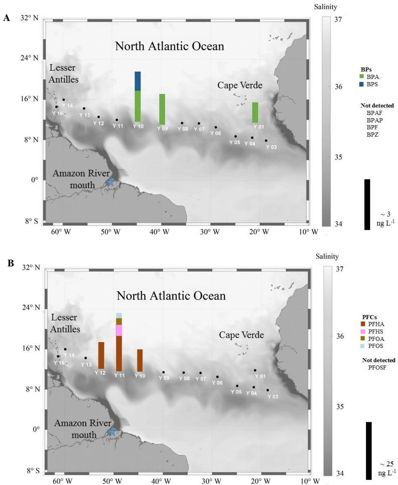
Fig. 3: Concentrations (in ng L -1 ) of the individual BPs (A) and PFCs (B) detected at sampling stations Y 01 - Y 16. Monthly average salinity distribution in the surface waters of the tropical North Atlantic in October 2017 is indicated as well as the Amazon River mouth (blue star).
