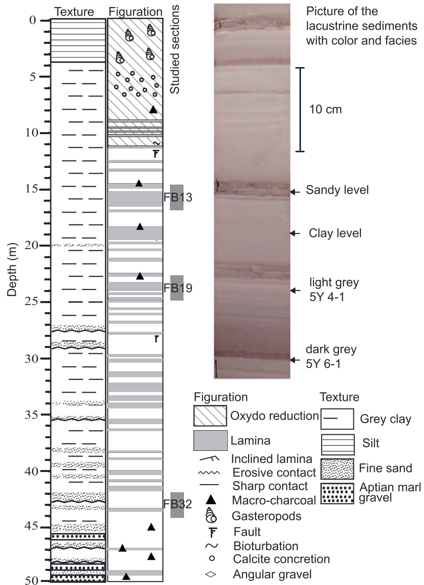
Figure 6. Schematic sedimentary log of Cassis paleolake. A right-color photograph of sediment is shown with color indication (Mussel code). The paleoenvironmental interpretation in the present study only concerns the nonoxidized sediments. The location of the three studied U-channels in the sedimentary sequence is also indicated.
