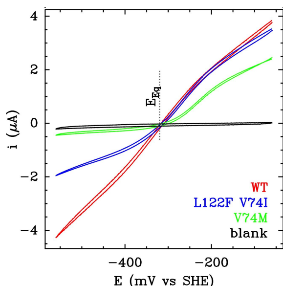
Figure 11 Bidirectional electrocatalysis by the WT (red), L122F-V74I (blue), and V74 M (green) forms of D. fructosovorans [NiFe] hydrogenase. At the equilibrium potential, the rates of oxidation and reduction exactly cancel each other and the current is zero. The blank was recorded with no adsorbed enzyme. Reprinted from ref 7 , with permission.
