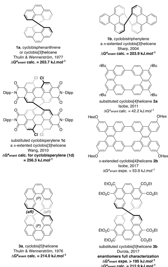
Figure 1. Known cyclobis[ n ]helicenes and scope of the present study (in bold).
