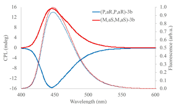
Figure 5. Circularly polarized luminescence (CPL) spectra of (P,aR,P,aR) - 3b (blue) and (M,aS,M,aS) - 3b (red). The dashed lines are the fluorescence emissions. Concentration = 8 \mu\text{mol L}^{-1} in dichloromethane. The excitation wavelength was 315 nm.
