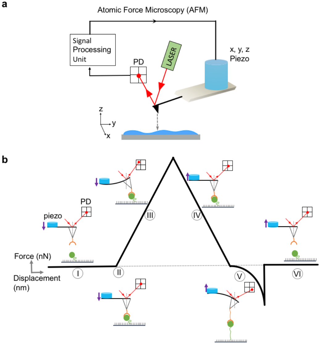
Figure 1. A schematic of the AFM and force measurement a . Schematic illustration of the fundamental components of an AFM device with working principles. b . A schematic photodetector signal of the cantilever deflection recorded during a biomolecular force spectroscopy curve together with the corresponding position of cantilever and surface.
