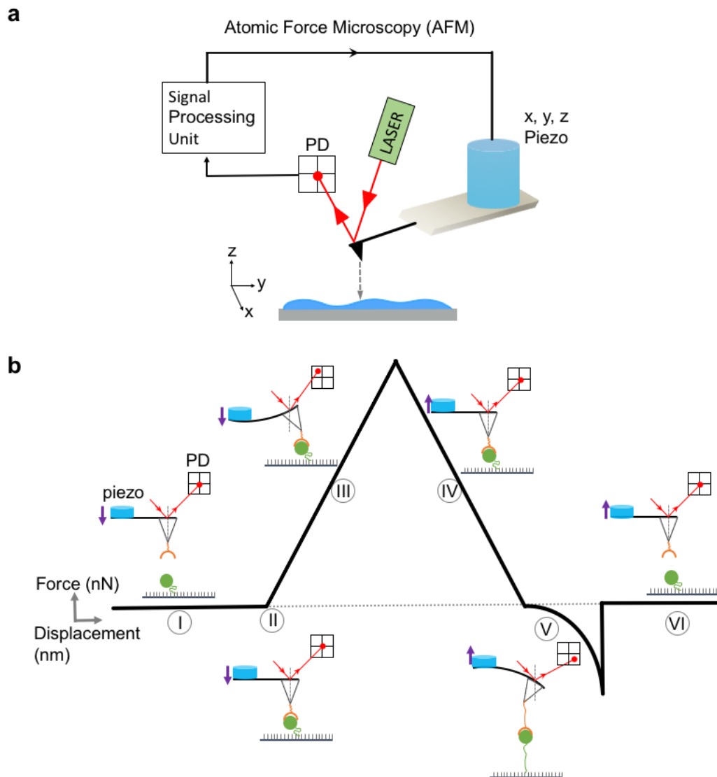
Figure 1. A schematic of the AFM and force measurement a. Schematic illustration of the fundamental components of an AFM device with working principles. b. A schematic photodetector signal of the cantilever deflection recorded during a biomolecular force spectroscopy curve together with the corresponding position of cantilever and surface.
