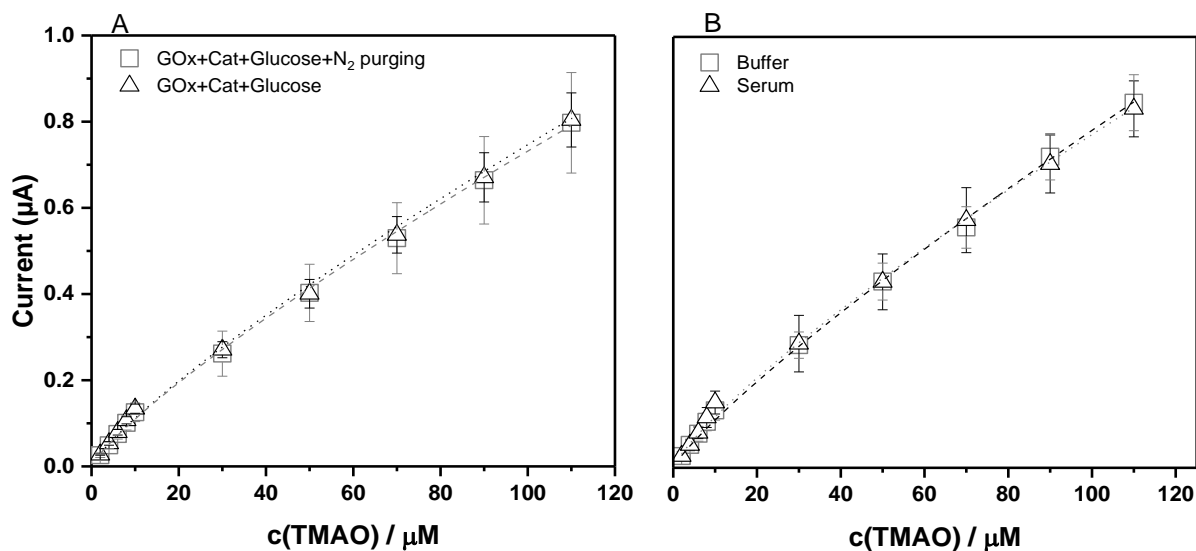
Figure 5. Graph of the current response versus the concentration of TMAO A) N 2 purging additional on the O 2 removal system (squares) and without purging (triangles). B) in undiluted serum (triangles) and in buffer solution (squares). Potassium phosphate buffer 100 mM pH 6.5; Range of TMAO 2-110 \mu\text{M} ; Methyl viologen 250 \mu\text{M} ; GOx 8 U, Cat 200 U and glucose 50 mM, (n=3 electrodes)
