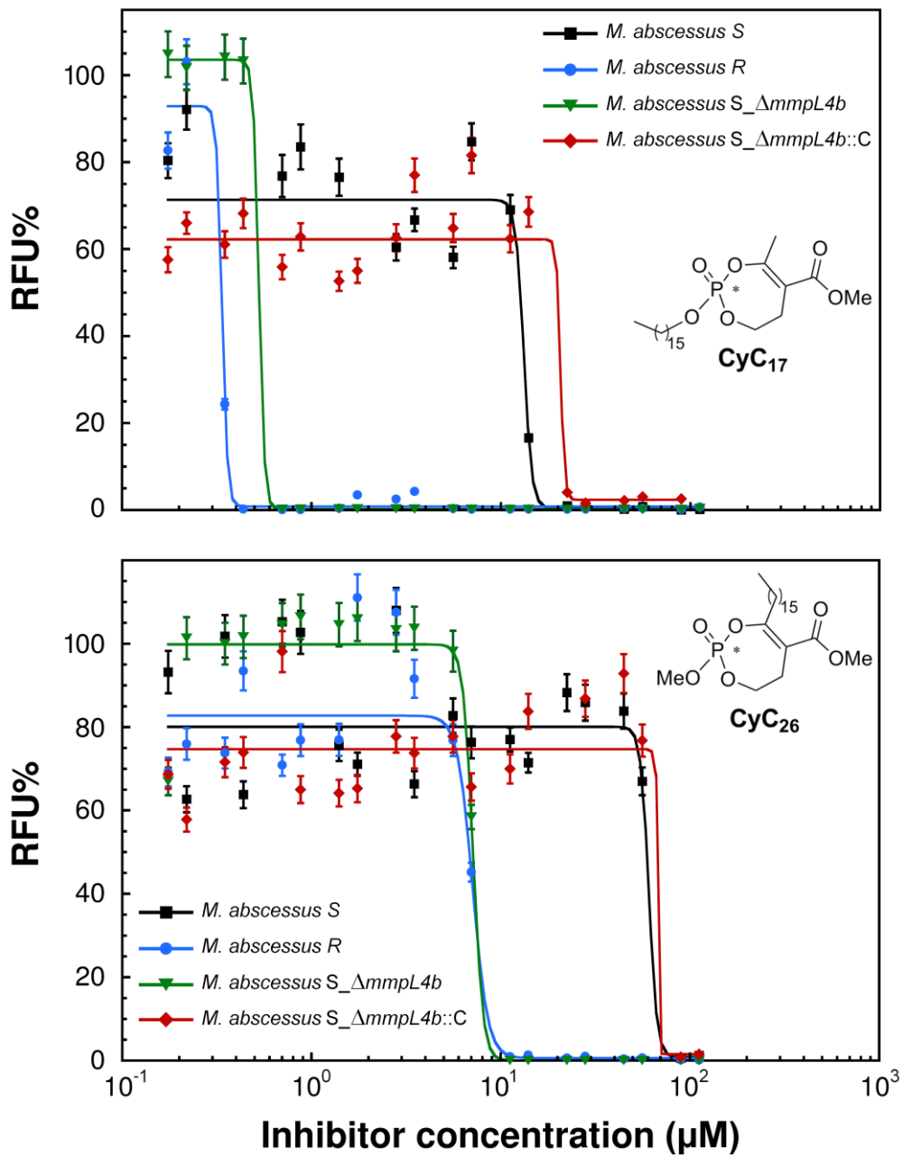
Figure 2. Dose-response activity of CyC 17 and CyC 26 against M. abscessus S, \Delta mmpL4b mutant ( M. abscessus S_ \Delta mmpL4b ), \Delta mmpL4b complemented ( M. abscessus S_ \Delta mmpL4b ::C), and M. abscessus R strains replicating in broth medium, expressed as normalized relative fluorescence units (RFU%). For each concentration, data are means \pm SD of at least two independent assays performed in duplicate (CV% <5%).
