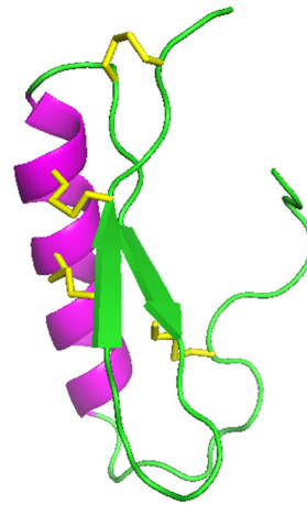
Figure 9. Three-dimensional structure of the As-ABF-alpha (PDB ID: 2D56): In green, antiparallel β-sheets; in purple, α-helix; and in yellow, disulfide bridges [35]. Picture generated using PyMOL (TM) 2.3.2 software ( www.pymol.org ).
