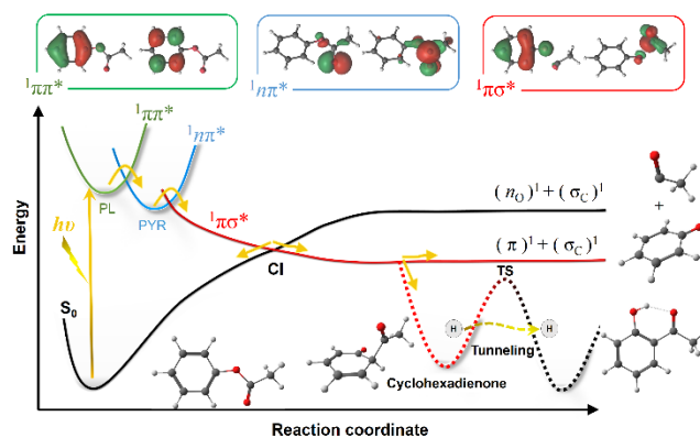
Figure 1. Schematic overview of the three-state model for PFR applied to PA. The insets show the main orbital transitions of the states involved in the PFR. Along the solid lines, the OC–O bond distance is the main reaction coordinate. Along the dashed curve, the hydrogen shift between the oxygen and ortho carbon is the main reaction coordinate.
