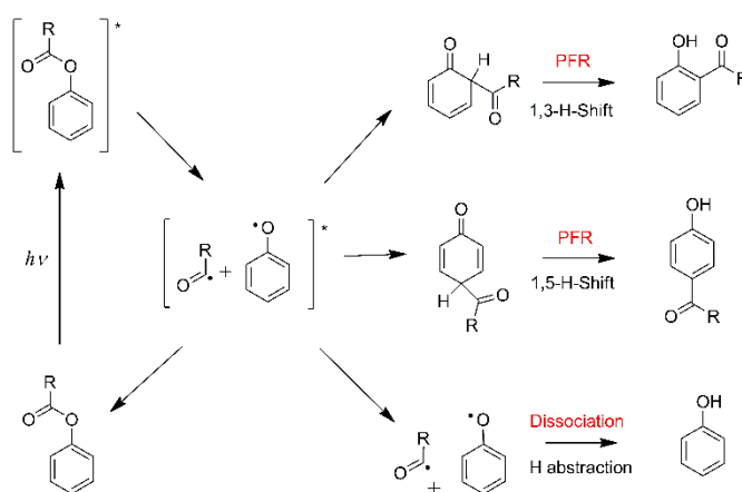
Scheme 1. General scheme of Photo-Fries rearrangement. For phenyl acetate, R = methyl.
