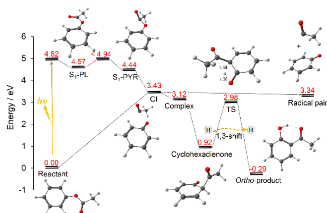
Figure 2. MS-CASPT2 energies along the Photo-Fries rearrangement of PA. CI: Conical intersection; TS: Transition state.
