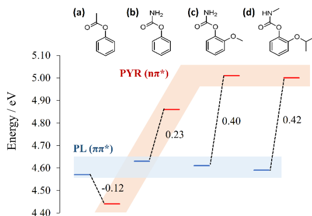
Figure 4. Energies of the planar ^1(\pi\pi^*) and pyramidal ^1(n\pi^*) S_1 minima of (a) phenyl acetate, (b) phenyl carbamate, (c) ortho -methoxyphenyl carbamate, and (d) 2-isopropoxyphenyl methylcarbamate (Propoxur) in the gas phase. Computed with CASPT2//CASSCF.
