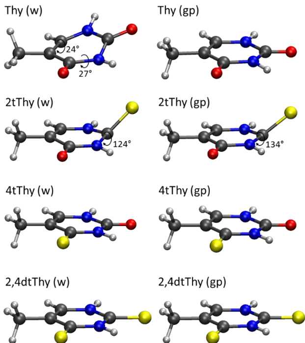
Figure 4. S_1 optimized structures of Thy and its thio-derivatives in water (w) and in the gas phase (gp).
