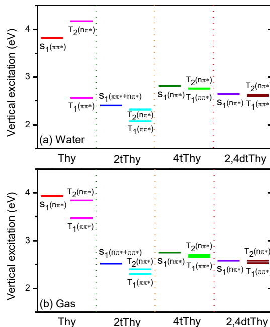
Figure 5. Singlet and triplet state distributions at the S_1 minimum. CASPT2 using TDDFT geometries optimized in (a) water and (b) the gas phase.
