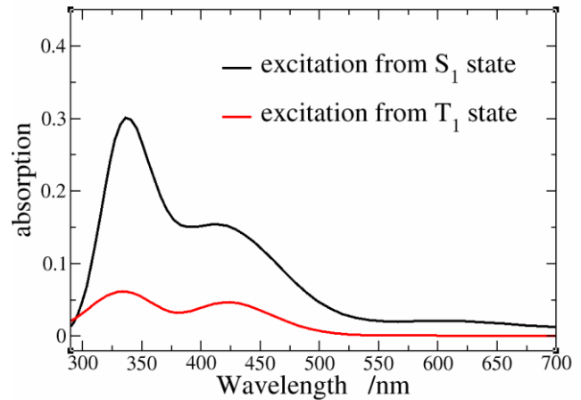
Figure 6. Absorption spectra from the T_1 and S_1 minima of Thy.
