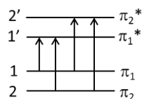
Scheme 1. 4/4 minimum model for \pi\pi^* excitation of Thy and its thio-derivatives.
