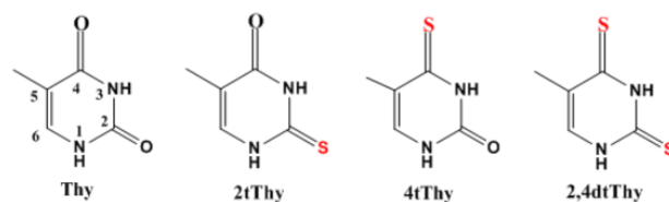
Figure 1. Structure of the molecules investigated in this paper: 2-thiothymine (2tThy), 4-thiothymine (4tThy), and 2,4-dithiothymine (2,4dtThy). Throughout the text, equivalent notation will be used for thymidine (Thd) and uracil (Ura).
