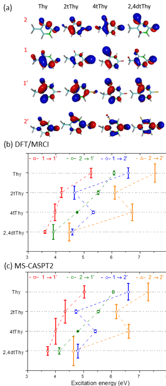
Figure 3. (a) The two occupied \pi orbitals (MO 1 and MO 2) and unoccupied \pi^* orbitals (MO 1' and MO 2' ) involved in the excitations of Thy, 2tThy, 4tThy, and 2,4dtThy, from DFT calculations. (b) Comparison of different excitations including excitation energy and oscillator strength (given by the bars size) among the four molecules for DFT/MRCI. (c) The same as in (b) for MS-CASPT2.
