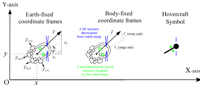
Fig. 1. Description of the simulated robot . The hovercraft is equipped with two side and two rear thrusters that acts upon the forward thrust via the sum of the rear thrusters F_{RT1} + F_{RT2} , upon the yaw torque via the difference between the left and right rear thrusters F_{RT1} - F_{RT2} and upon the side thrust via the difference between the left and right thrusters F_{LT1} - F_{LT2} . The sound sensors are mounted on the robot body ( Green circles ) while the right and left gazes of optic flow sensor are uncoupled from the robot's body ( Blue lines ). In the plots of the simulated trajectories, the robot is represented by the symbol shown to the right.
