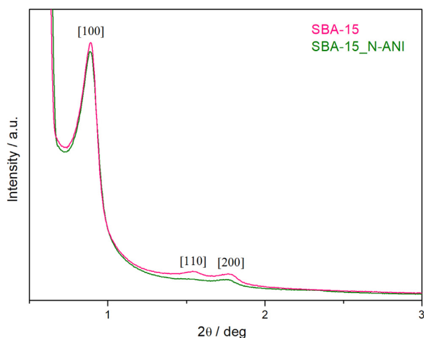
Fig. 2. Small-angle XRD diffractogram of the mesoporous silica SBA-15 and SBA-15_N-ANI.
