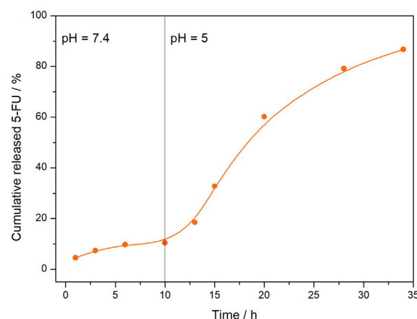
Fig. 8. The release profile of 5-FU from the solid SBA-15_N-ANI_5-FU_β-CD before and after adjusting pH to 5.
