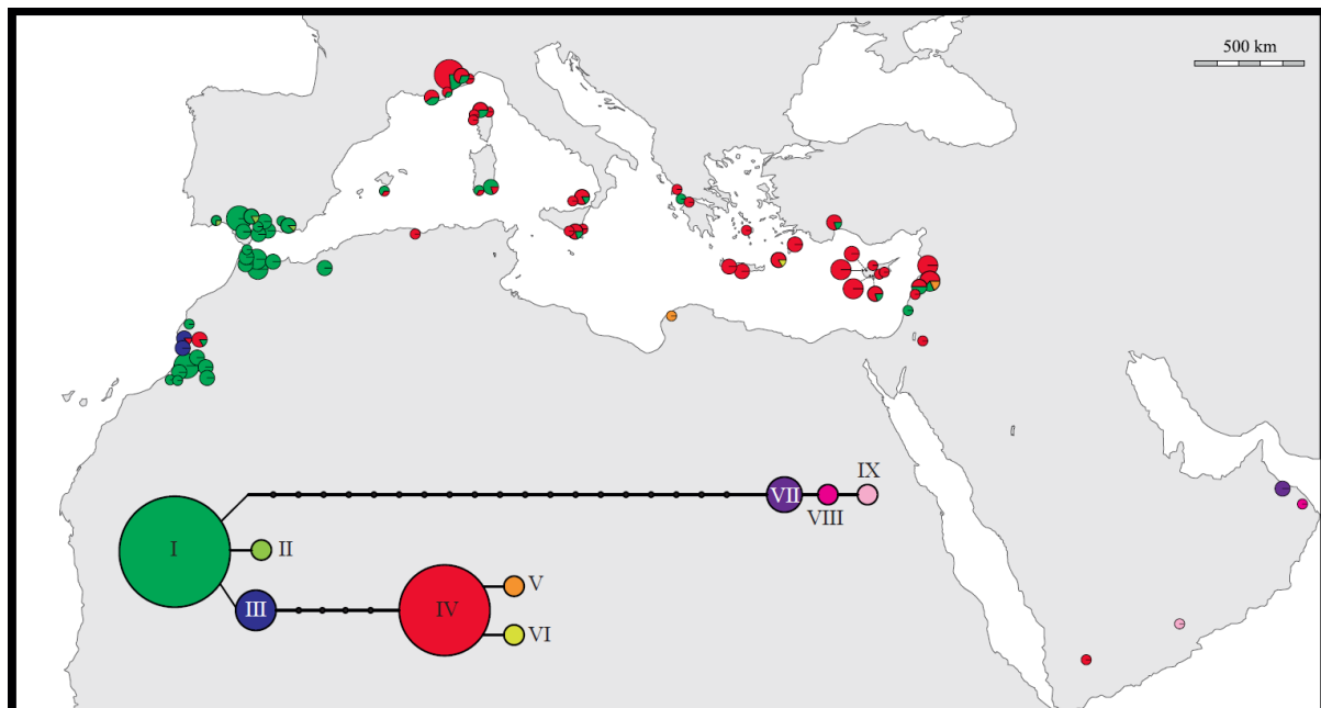
Figure 2: Geographic distribution of the plastid haplotypes identified in Ceratonia siliqua (I to VI) and C. oreoethauma (VII to IX). In the haplotype network, the size of the circles is representative of sample size. Four markers were sequenced to obtain these haplotypes for a total of 1472 bp.
