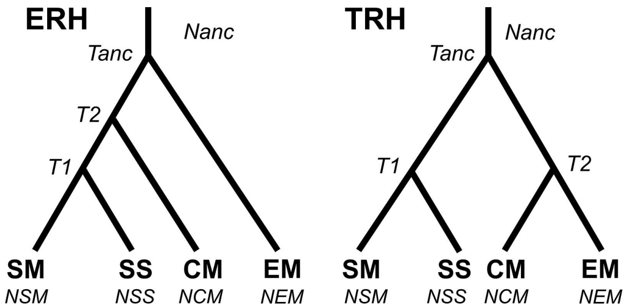
Figure 1: Candidate models for the phylogeography of Ceratonia siliqua . ERH is the eastern refugium hypothesis and TRH the two refugia hypothesis. SM, SS, CM and EM correspond to the Southern Morocco, South Spain, Central Mediterranean and Eastern Mediterranean genetic groups, respectively.
