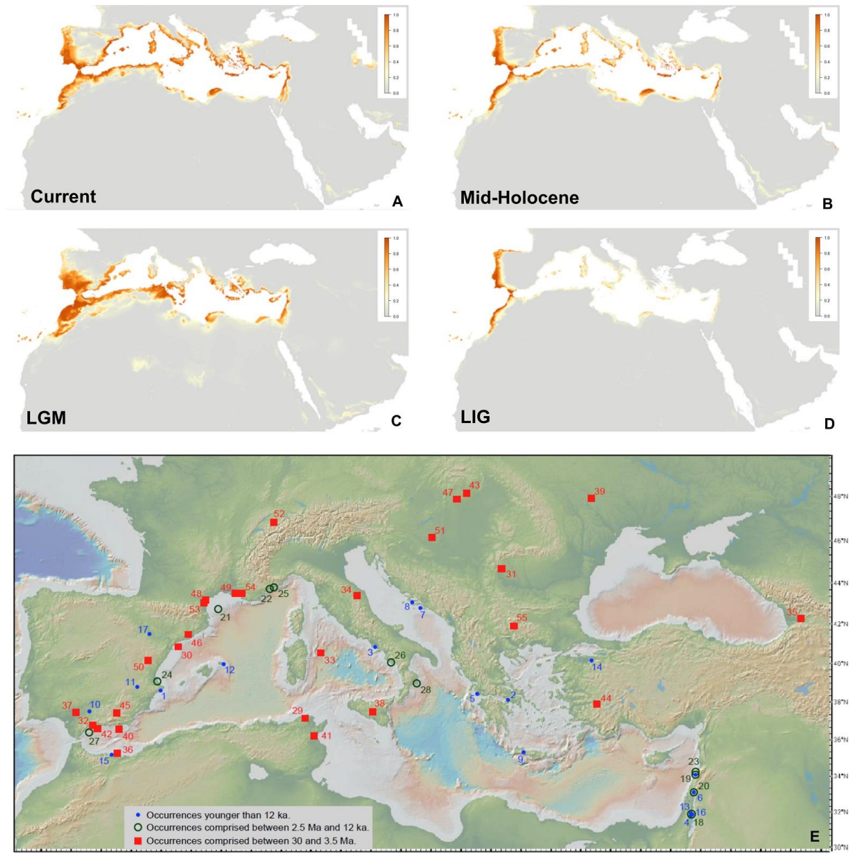
Figure 5: Species distribution modelling of the carob in four periods (A, Present; B, Mid-Holocene; C, Last Glacial Maximum (LGM); D, Last Inter-Glacial (LIG)), and E, Map of palaeobotanical data of Ceratonia from Oligocene to Middle Ages (macroremains and pollen grains). Numbers correspond to the input order of data in Table S2.5 from the youngest (No.1, Middle Ages) to the oldest data (No.55, Early Oligocene).
