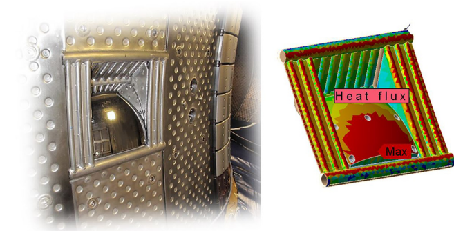
Fig. 3. Left: Mirror mounted in the inner wall of WEST - Right: calculated heat flux deposition pattern from plasma radiation (max = 130 kW/m 2 ).
