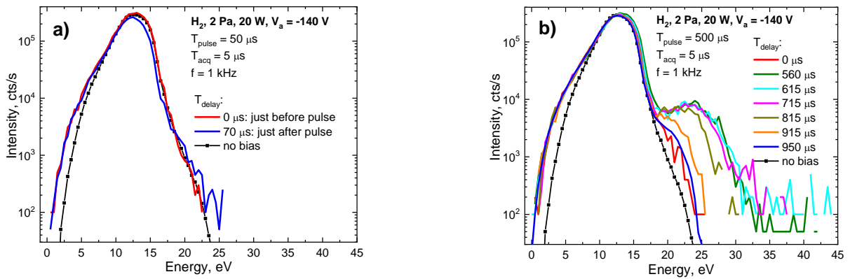
Figure 5: PIEDF of \text{H}_3^+ with (a) T_{\text{pulse}} = 50 \mu\text{s} (b) T_{\text{pulse}} = 500 \mu\text{s} and T_{\text{acq}} = 5 \mu\text{s} for various values of T_{\text{delay}} compared with the \text{H}_3^+ PIEDF in the absence of applied bias (symbols). Plasma parameters: 2.0 Pa of \text{H}_2 , P_{\text{RF}} = 20 \text{ W} , V_a = -140 \text{ V} , molybdenum clamp.
