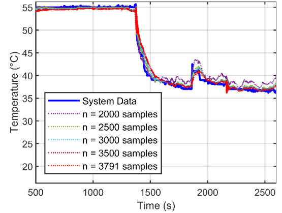
Figure 6: Estimations generated by multiple ARMAX RLS models with different sample numbers in their training sets against system measurements.
