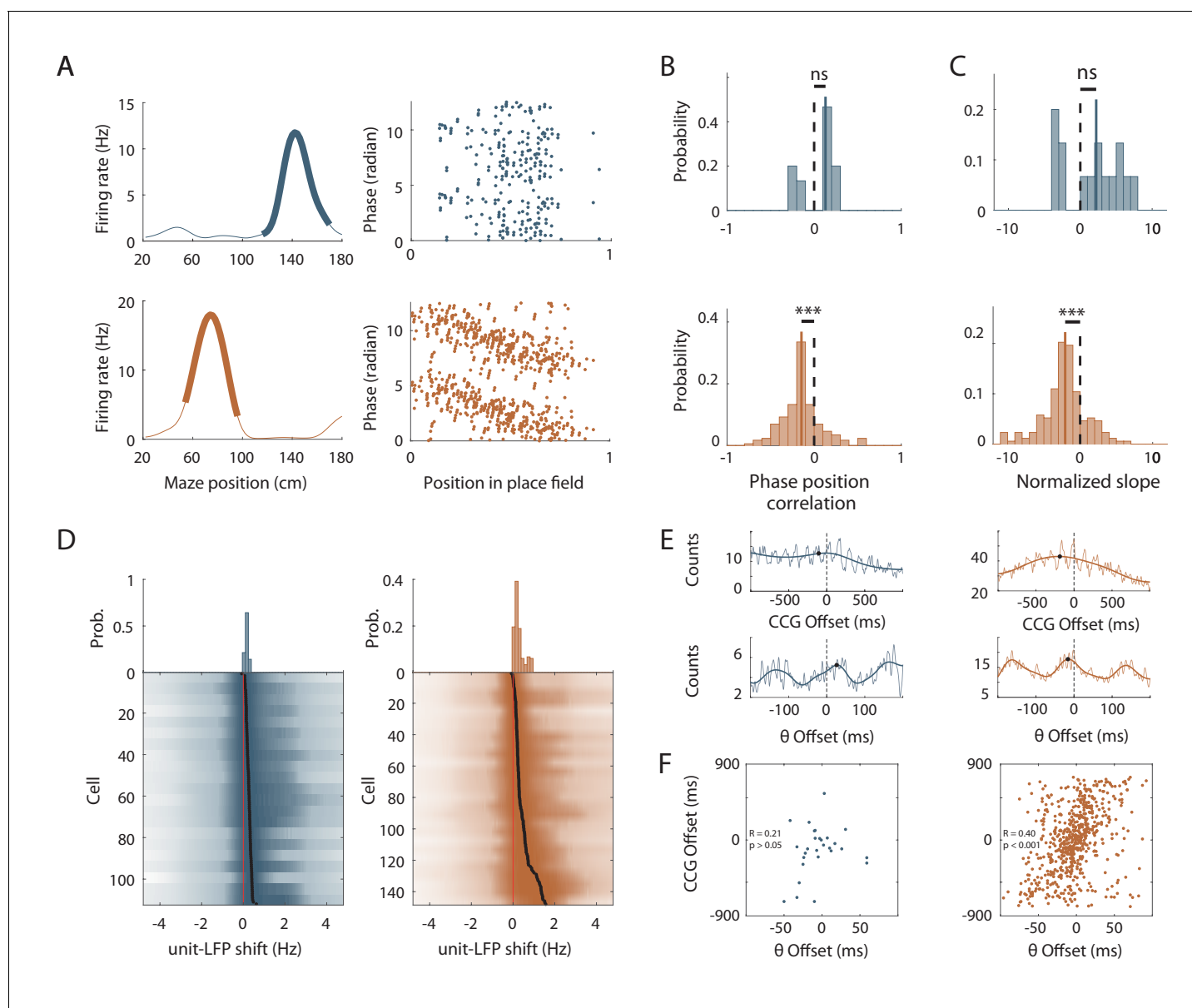
Figure 7. Effects of local cues on hippocampal temporal coding resolution. (A) Left: Mean firing rate maps of representative CA1 place cells with place fields highlighted by a bold line (left) recorded in the maze without objects (top, only spatially stable trials see Materials and methods section) and with objects (bottom). Right: spikes phase (radian) versus position in the corresponding place fields. (B–C) Distribution of significant phase position correlation (B) and slopes (C) in the condition without objects (top; correlation) and with objects (bottom). The median of the distribution is indicated by a bold line and 0 by a dotted line. (D) Color-coded cross-correlogram between the power spectra of neuronal spikes and LFP for each theta-modulated cell recorded on the maze without (bottom left, blue) and with (bottom right, orange) objects. Black dots indicate the maximum of each cross-correlation. Each cross-correlation is normalized by its maximum. Top: Distribution of the maximum cross-correlations used to quantify the frequency shift for all the cells. (E) Examples of cross-correlograms computed for two pairs of place cells with overlapping place fields at the behavioral (top) or theta time scale (bottom, see Materials and methods) in order to quantify Cross-Correlogram (CCG) and theta Offsets respectively in no object (blue; left) or object (orange; right) conditions. (F) Relationship between ‘CCG’ and ‘theta’ offsets in the cross-correlograms of all the spikes in overlapping place fields of neuron pairs recorded in no object (top; blue) and object condition (bottom; orange).
