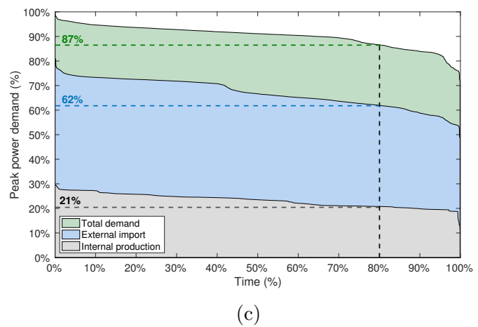
Figure 7: Refinery blueprint - electrical energy profile with main power flows (a), electrical consumptions breakdown (b) and load duration curve (c)
