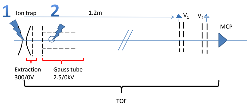
Figure SI-1: Scheme of the experimental setup. The two regions where the laser interacts with the ion packet are 1) in the cold trap, and 2) in the gauss tube.
