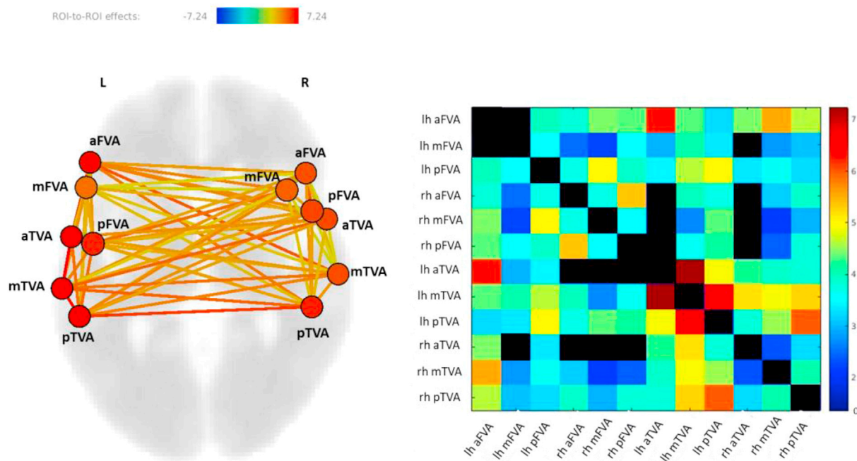
Fig. 2. Functional connectivity within the voice perception network. Axial view of the ROI-to-ROI FC (left; p-FDR seed-level corrected < 0.05 ) and connectivity matrix reporting t-values for the contrast V vs NV (right). The black squares in the connectivity matrix are used to visualize non-significant correlations at p-FDR seed-level corrected < 0.05 or same-seed correlation. Note that both colorbars report t-test values between two seeds (DOF = 89), but the minimum value in the left colorbar is negative ( -7.24 ) while in the connectivity matrix is 0. Lh = left hemisphere; rh = right hemisphere.
