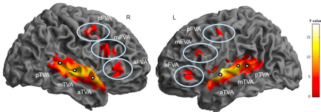
Fig. 1. Random effect analysis in 92 subjects. Suprathreshold clusters showing higher activation for the contrasts V vs NV ( N = 92 , p < 0.05 FWE voxel-level corrected, extent threshold = 0 \text{ mm}^3 ). The black-light blue points represent approximate location of the six TVAs. The frontal clusters where individual FVAs were defined are instead in the light blue circles (a = anterior; m = middle; p = posterior).
