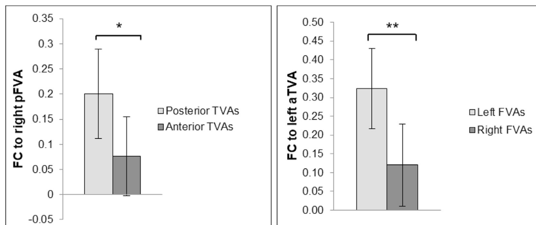
Fig. 3. Bar graphs representing differences in ROI-to-ROI FC between posterior and anterior TVAs (left graph) and between left and right FVAs (right graph). Error bars represent 95% confidence intervals (*p-FDR corrected (two-sided) < 0.05; **p-FDR corrected (two-sided) < 0.001).
