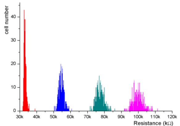
Figure 15. R_{ON} distributions versus cell variability ( \sigma_{\text{Variability}} = 20\% ) after 300 runs (SET states)
