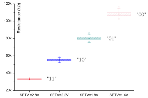
Figure 14. R_{ON} distribution box-plots versus cell variability ( \sigma_{\text{Variability}} = 15\% ) after 300 runs (SET states)
