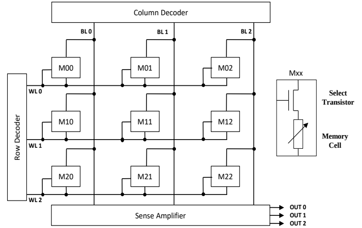
Figure 8. 3×3 OxRAM elementary memory array
