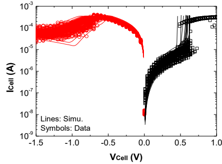
Figure 3. Measured and corresponding simulated I-V characteristic obtained from TiN/Ti/HfO 2 /TiN devices showing strong variation on R_{\text{LRS}} and R_{\text{HRS}}
