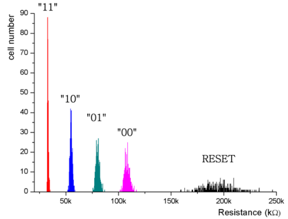
Figure 13. R_{ON} and R_{OFF} distributions versus cell variability ( \sigma_{\text{Variability}} = 15\% ) after 300 runs (SET and RESET states)
