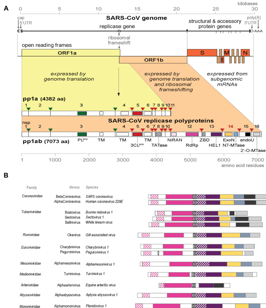
FIGURE 1 | (A) Outline of the CoV genome organization and expression strategy. Depicted are the SARS-CoV genome and its 14 open reading frames (ORFs), i.e., the replicase ORFs 1a and 1b, the four common CoV structural protein genes (S, E, M, and N) and the ORFs encoding “accessory proteins.” The bottom half of the scheme summarizes the proteolytic processing and domain organization of the pp1a and pp1ab replicase polyproteins, the latter being produced by -1 ribosomal frameshifting. The nsp3 (PLpro, green) and nsp5 (3CLpro, red) proteases and their cognate cleavage sites are indicated in matching colors. The resulting 16 cleavage products (non-structural proteins, nsps) are indicated, as are the conserved replicase domains that are relevant for this review. See main text for references on nsp functions. Domain abbreviations and corresponding nsp numbers: PLpro, papain-like proteinase (nsp3); 3CLpro, 3C-like or main proteinase (nsp5); TM, transmembrane domain (nsp3, nsp4, and nsp6); NIRAN, nidovirus RdRp-associated nucleotidyl transferase (nsp12); RdRp, RNA-dependent RNA polymerase (nsp12); ZBD, zinc-binding domain (nsp13); ExoN, 3'-to-5' exoribonuclease (nsp14); N7-MTase, N7-guanine methyl transferase (nsp14); endoU, uridylylate-specific endoribonuclease (nsp15); 2'-O-MTase, 2'-O-methyl transferase (nsp16); UTR, untranslated region. (B) Comparison of the predicted domain organization in the replicase polyprotein of selected members of the nine families currently classified within the order Nidovirales (ICTV release 2018b). Adapted from Bukhari et al. (2018), with permission. Domains were predicted using HHPred-search (Soding, 2005; Zimmermann et al., 2018); for abbreviations see the legend to panel A. Genbank accession numbers of sequences used: SARS-coronavirus (AY274119.3); Human coronavirus 229E (AF304460.1); Bovine nidovirus 1 (KM589359.1); Sectovirus 1 (KX883637.1); White bream virus (DQ898157.1); Gill-associated virus (AF227196.1); Charybnavirus 1 (KX883628.1); Paguronivirus 1 (KX883627.1); Alphamesonivirus 1 (DQ458789.2); Turrinivirus 1 (KX883629.1); Equine arteritis virus (X53459.3); Aplysia abyssovirus (NC_040711.1); Planidovirus 1 (MH933735).
