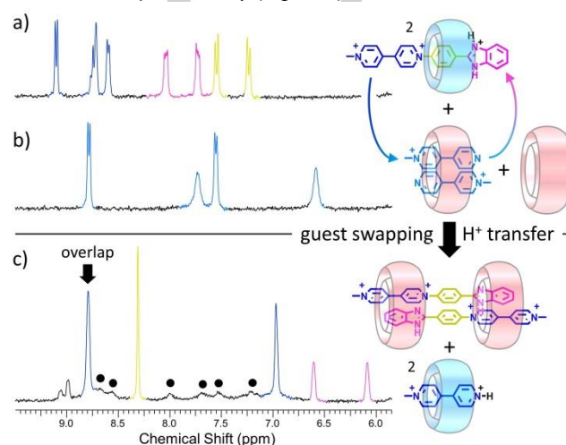
Figure 6. Excerpts of the aromatic region of 1 H NMR spectra for a) a mixture of V-P-I 2+ and CB[7], b) MPP 1+ and CB[8] and c) the mixture of solutions corresponding to a) and b) showing signals assigned to the formation of V-P-I 2+ •CB[8] 2 and of MPPH 2+ •CB[7] (signal overlap, see text) and illustrating the simultaneous host/guest swapping and proton transfer (● stands for residual signals from V-P-I 2+ •CB[7]).
