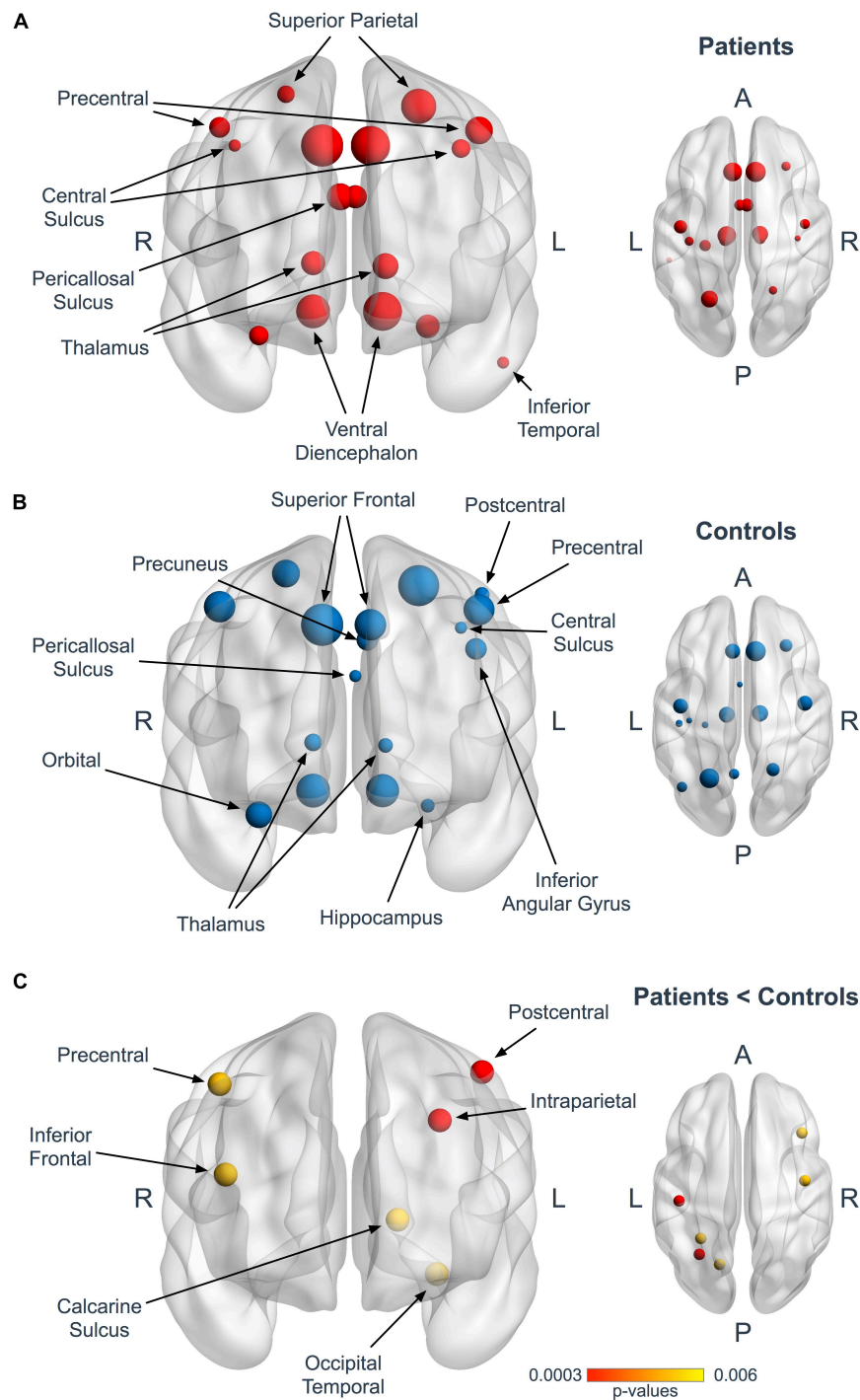
FIGURE 2 | Hubs in ALS patients and controls. Panels (A,B) represent coronal and axial views illustrating the hubs in patients (A, red) and controls (B, blue) . The size of the nodes is proportional to their degree values. Panel (C) shows the 6 nodes with significantly reduced mean degree in patients at the Bonferroni corrected threshold (red, p < 0.0003 ) and at the 1/n exploratory threshold (yellow, p < 0.006 ).
