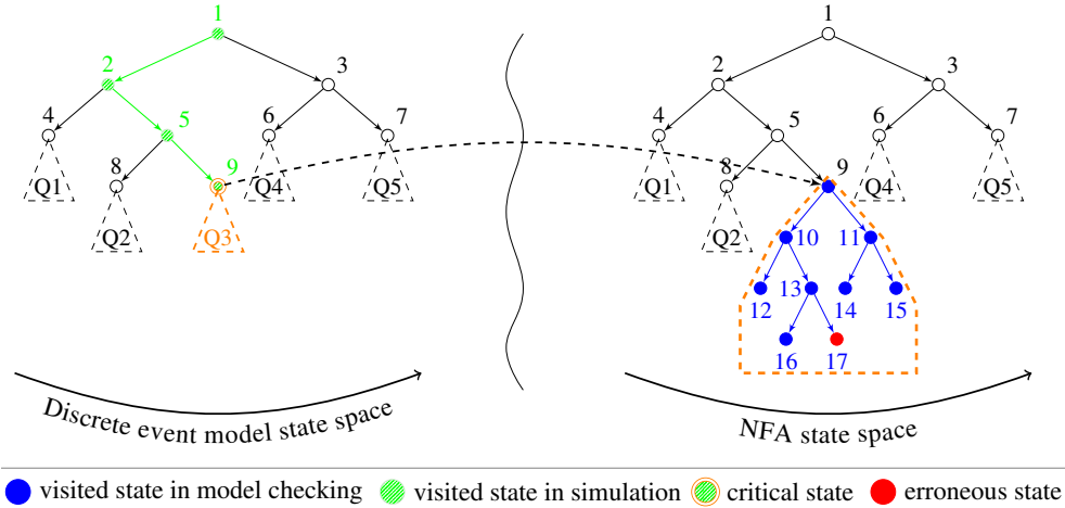
Figure 1: Illustration of the state space exploration with the combined approach.
