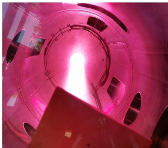
Figure 17: Photo of the plasma jet ( H_\alpha plasma emission) emitted by the 3 kW Helicon in the cylindrical diffusion chamber of the RAID testbed. Axial magnetic field of \sim 10 \text{ mT} .
