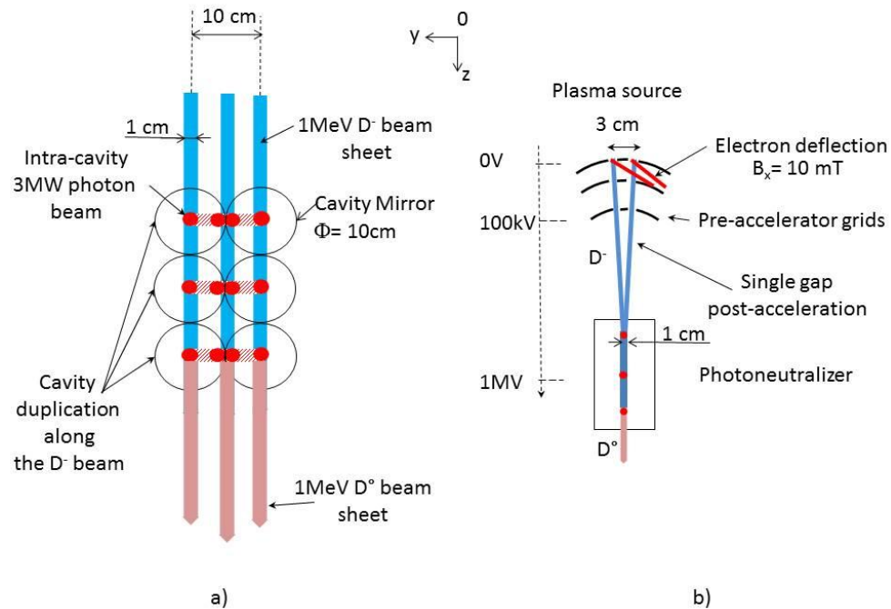
Figure 2: a) Top view: Duplication of three optical independent 3MW cavities along three \text{D}^- beam sheets. b) Pre and post acceleration principle for one \text{D}^- beam sheet (Top view).
