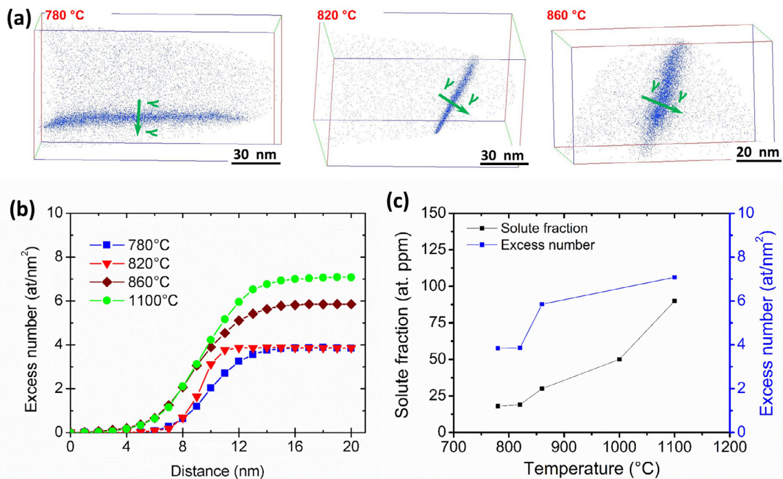
Fig. 3. (a) Reconstructed APT volumes after three soaking temperatures. (b) Boron integral profiles measured by APT giving the excess numbers in \text{at}/\text{nm}^2 at \gamma\text{GB} s for four different soaking temperatures. (c) Boron concentrations in solid solution measured in the grain center by nano-SIMS (black squares, left axis); and excess numbers at \gamma\text{GB} measured by APT (blue squares, right axis), as a function of soaking temperature. (For interpretation of the references to colour in this figure legend, the reader is referred to the web version of this article.)
