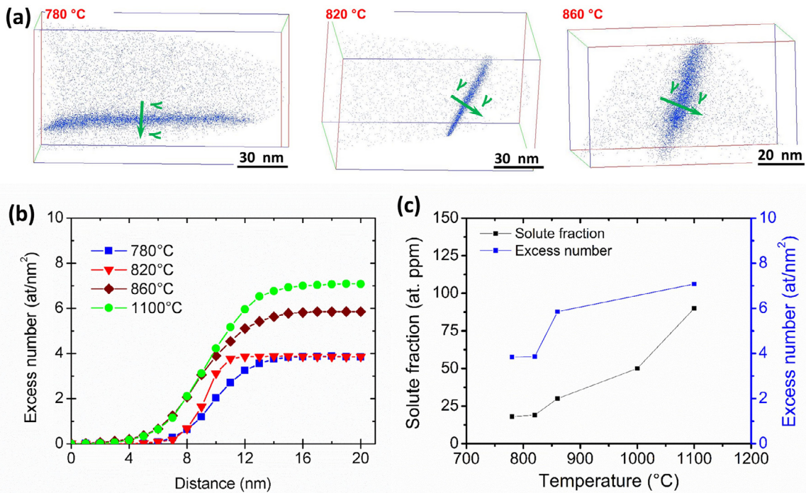
Fig. 3. (a) Reconstructed APT volumes after three soaking temperatures. (b) Boron integral profiles measured by APT giving the excess numbers in \text{at}\cdot\text{nm}^{-2} at \gamma\text{GB} s for four different soaking temperatures. (c) Boron concentrations in solid solution measured in the grain center by nano-SIMS (black squares, left axis); and excess numbers at \gamma\text{GB} measured by APT (blue squares, right axis), as a function of soaking temperature. (For interpretation of the references to colour in this figure legend, the reader is referred to the web version of this article.)
