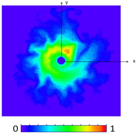
Figure 2.8: Distribution of the plasma density (normalized plasma density) at a given time for B=5 \text{ mT} , p=0.26 \text{ Pa} (linear scale, unit 2 \times 10^{18} \text{ m}^{-3} ).
