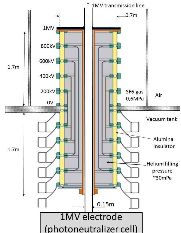
Figure 5.1: 1MV compact Bushing concept.
