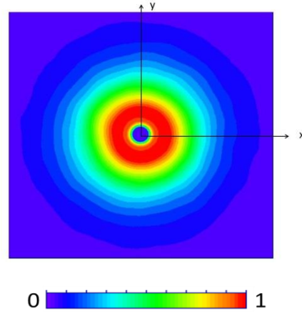
Figure 2.9: Time averaged distribution of the plasma density in the conditions of Fig. 2.8 (linear scale, unit 2 \times 10^{18} \text{ m}^{-3} ).
