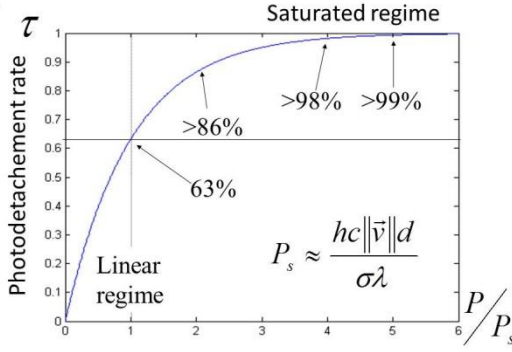
Figure 4.1: Photodetachment rate as a function of the relative photon power
