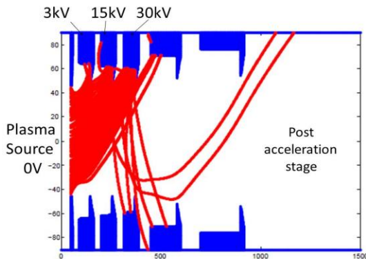
Figure 3.4: 3D trajectories of the co-electron in one pre-accelerating channel (top view of one slot) for a uniform magnetic field (normal to the plan of the figure) of 6 mT.
