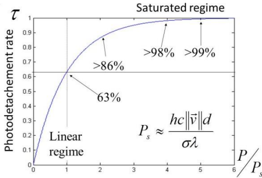
Figure 4.1: Photodetachment rate as a function of the relative photon power
