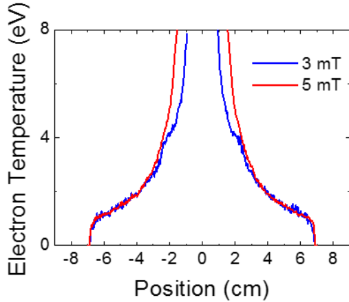
Figure 2.10: Radial distribution of the time averaged electron temperature.
