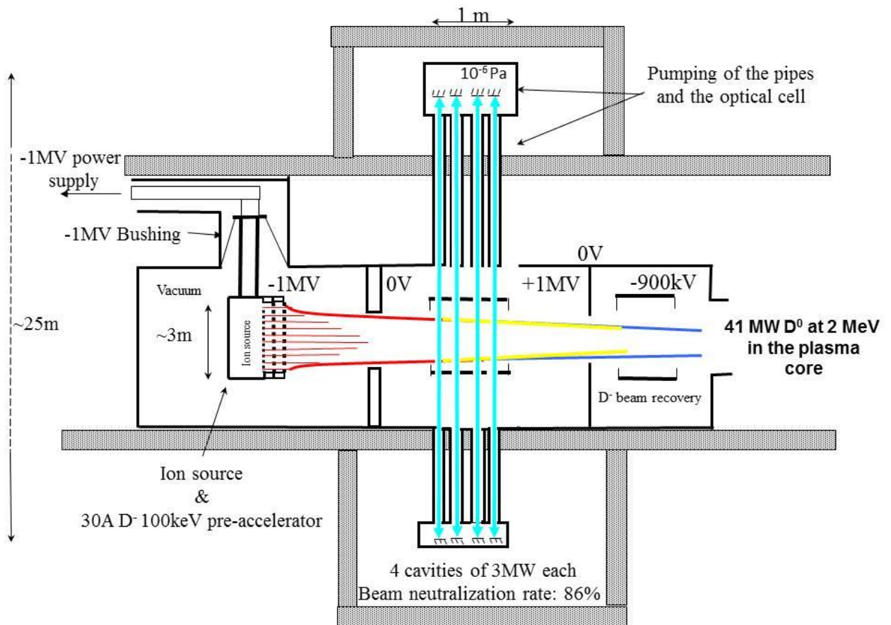
Figure 1.4: Side view of a 2MeV Siphore injector, with the source at -1MV and the photoneutralizer at +1MV; the ion source and pre-accelerator are sustained under vacuum polarized at -1MV and supplied by a vertical bushing. The photoneutralizer and recovery cells are sustained under vacuum by lateral Bushings (not shown on the figure) at +1MV and -900kV respectively.
