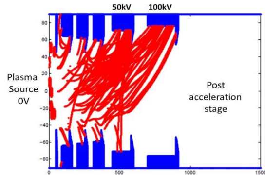
Figure 3.5: 3D trajectories of the stripped electron in one pre-accelerating channel for a magnetic field of 6 mT.
