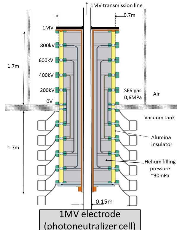
Figure 5.1: 1MV compact Bushing concept.
