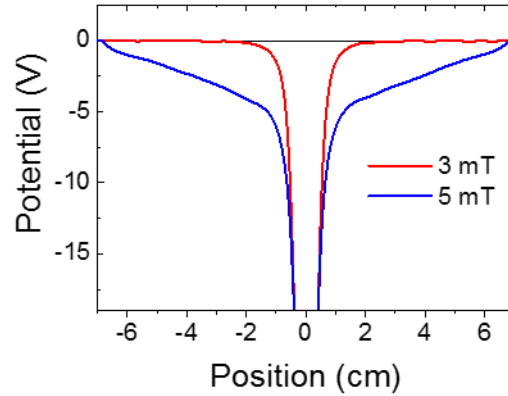
Figure 2.11: Radial distribution of the time averaged plasma potential.
