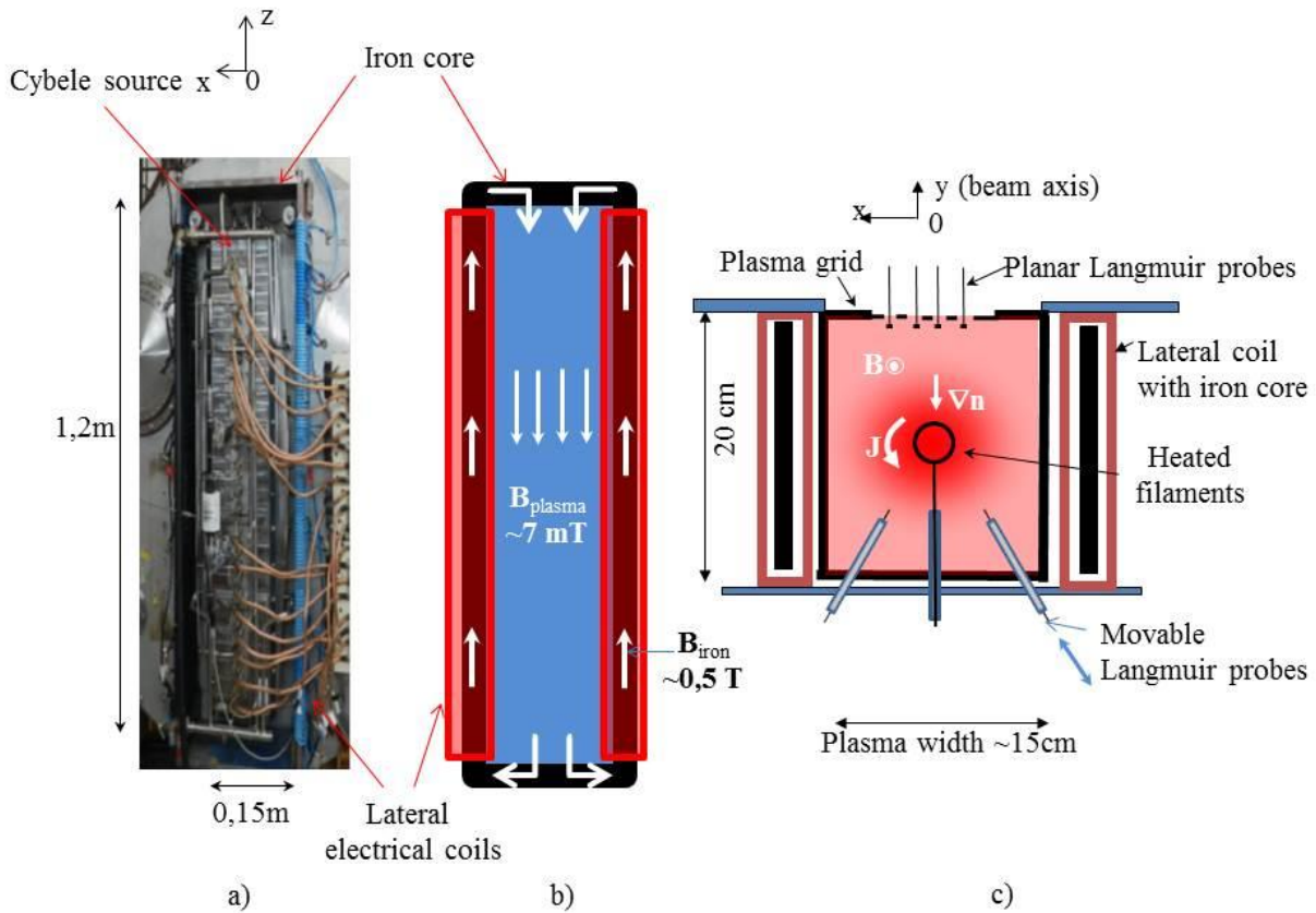
Figure 2.1: a) Photo of the Cybele source (back face) with the surrounding iron core and lateral coils; b) Schematic of the magnetic set up surrounding Cybele; c) Horizontal cross section of the source ; J is the plasma flow rotating around the cathode, and \nabla n is the gradient of the plasma kinetic pressure.
