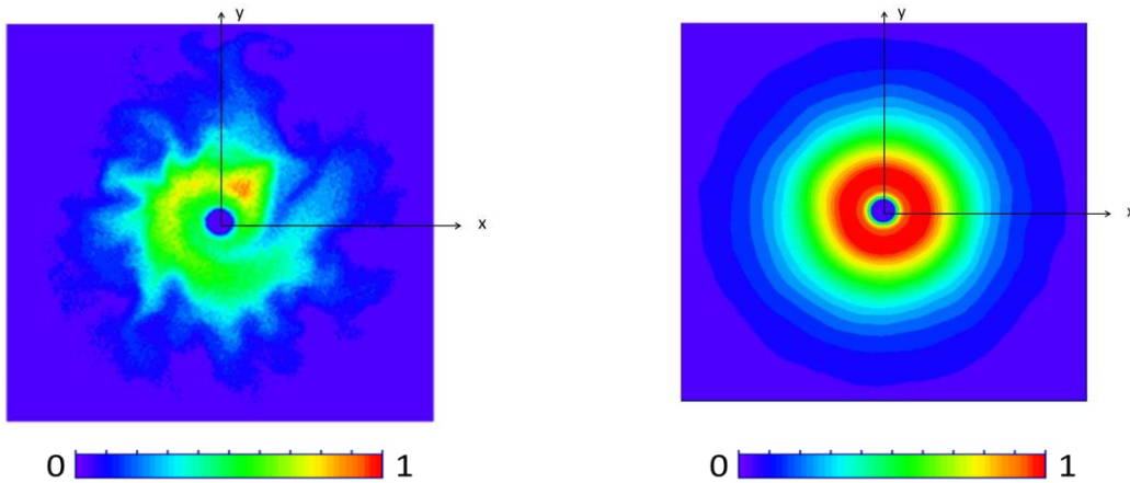
Figure 2.8: Distribution of the plasma density (normalized plasma density) at a given time for B=5 \text{ mT} , p=0.26 \text{ Pa} (linear scale, unit 2 \times 10^{18} \text{ m}^{-3} ).
