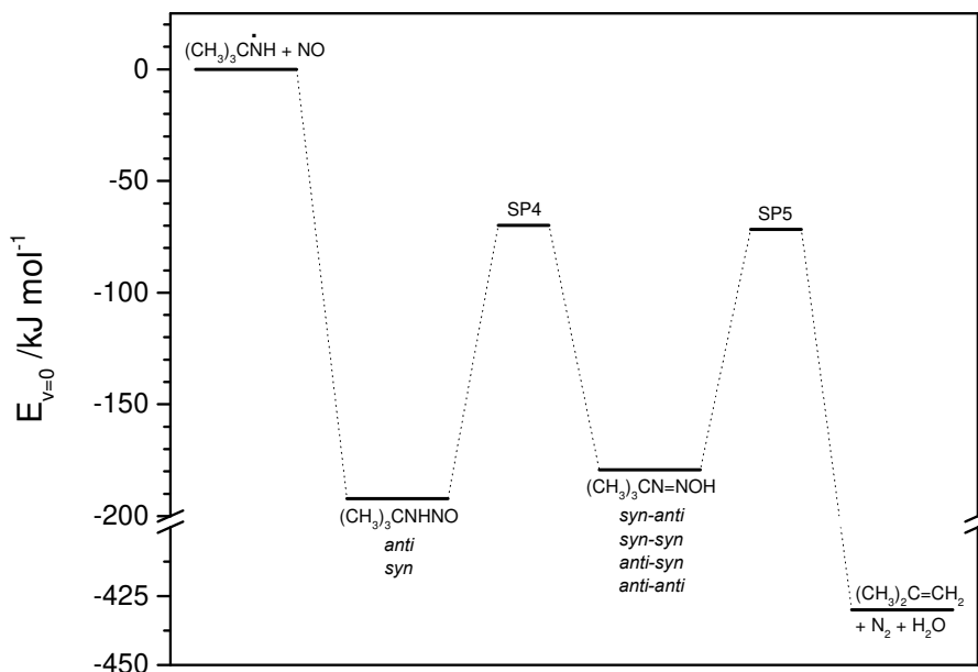
Figure 3. Stationary points on the simplified PES of the (\text{CH}_3)_3\dot{\text{C}}\text{NH} + \text{NO} reaction. Results are from CCSD(T*)-F12a/aug-cc-pVTZ//M06-2X/aug-cc-pVTZ calculations.
