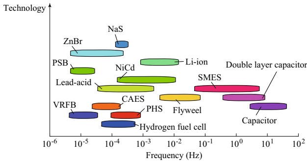
Fig. 9 Power Ragone chart in frequency plane
