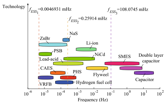
Fig. 16 Example of Selected ESS from the second Pareto-Front solutions
