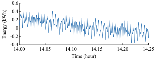
Fig. 8 ESS_h energy fluctuation over 15 minutes
