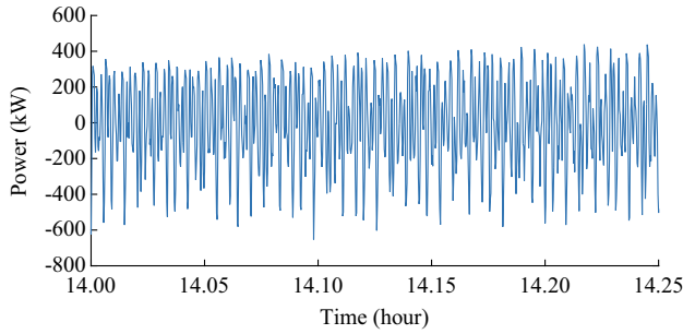
Fig. 7 ESS_h power fluctuation over 15 minutes
