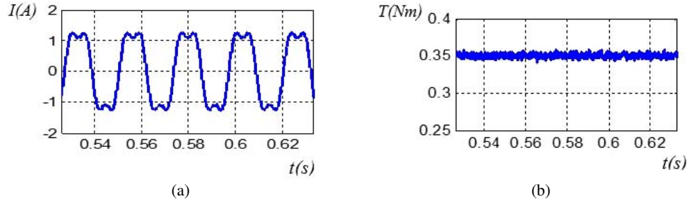
Fig. 7. Simulation results: (a) current in one phase of 5-phase machine; (b) torque
