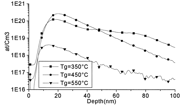
Fig. 3. Sb segregation in \text{Si}_{0.8}\text{Ge}_{0.2} . SIMS profiles for T_G = 350, 450 and 500^\circ\text{C} .
