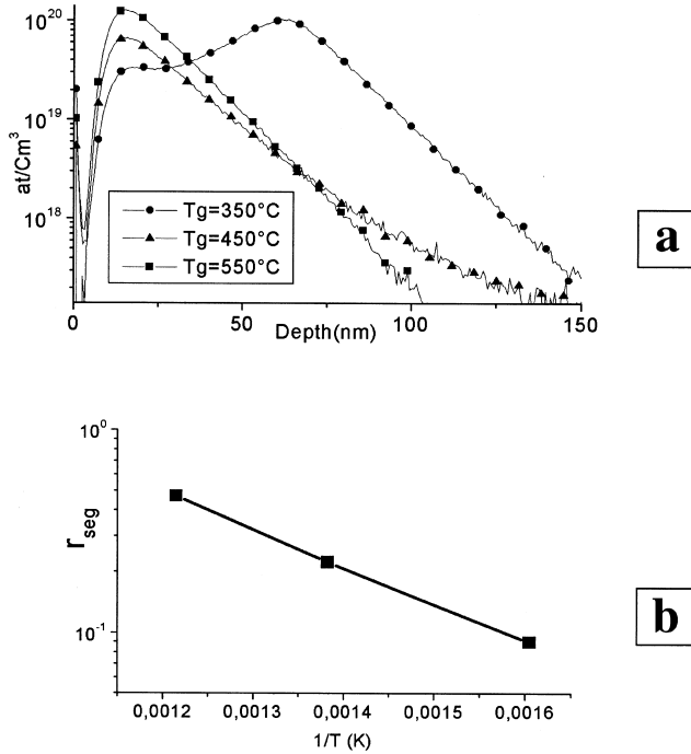
Fig. 2. (a) SIMS profiles of Sb in Si: T_G = 350, 450 and 550^\circ\text{C} . (b) Sb surface segregation coefficient ( r_{\text{seg}} ) measured in Si.
