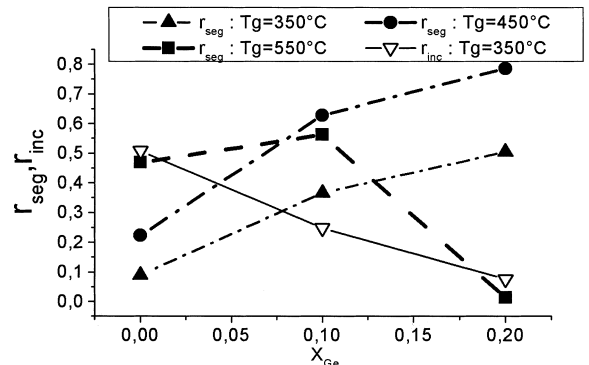
Fig. 4. Sb surface segregation ( r_{\text{seg}} ) and incorporation ( r_{\text{inc}} ) coefficients in \text{Si}_{1-x}\text{Ge}_x .
