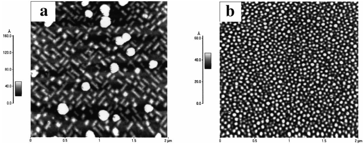
Fig. 5. AFM images 2 \times 2 \mu\text{m} . Growth of 8 ML of Ge (a) on Si(100) surface, (b) on 1 ML Sb pre-deposited on Si(100) surface.
