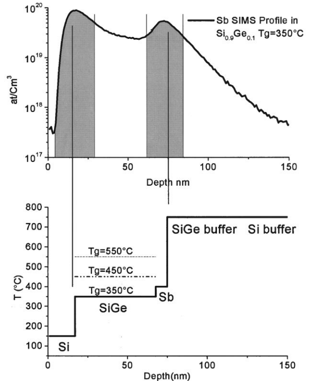
Fig. 1. Temperature sequences during growth.
