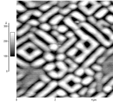
Fig. 4. AFM image of ripple-like islands elongated along \langle 100 \rangle and \langle 010 \rangle directions obtained in regime I for \text{Si}_{0.85}\text{Ge}_{0.15} ( h = 100 nm).
