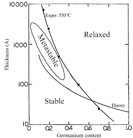
Fig. 1. Schematic view of the different states (strained, metastable and relaxed) of \text{Si}_{1-x}\text{Ge}_x alloys as a function of the thickness and of the Ge concentration.
