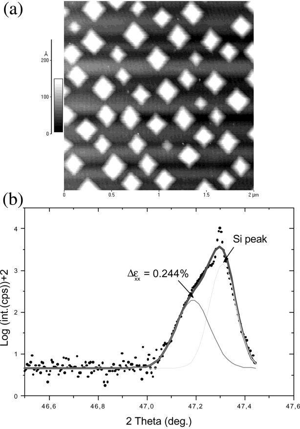
Fig. 6. (a) AFM image and (b) GIXRD spectrum of ‘hut’ islands stabilised during 18-h annealing at 550°C of a \text{Si}_{0.75}\text{Ge}_{0.25} ( h = 10 nm). An elastic relaxation \Delta\varepsilon_{xx} \sim 0.25\% was estimated.
