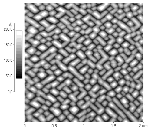
Fig. 5. AFM image of ‘hut’ islands elongated along \langle 100 \rangle and \langle 010 \rangle directions obtained in regime I for \text{Si}_{0.7}\text{Ge}_{0.3} ( h = 10 nm).
