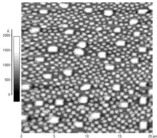
Fig. 3. AFM image of the bimodal size distribution of domes obtained in regime III for \text{Si}_{0.5}\text{Ge}_{0.5} ( h = 15 nm).
