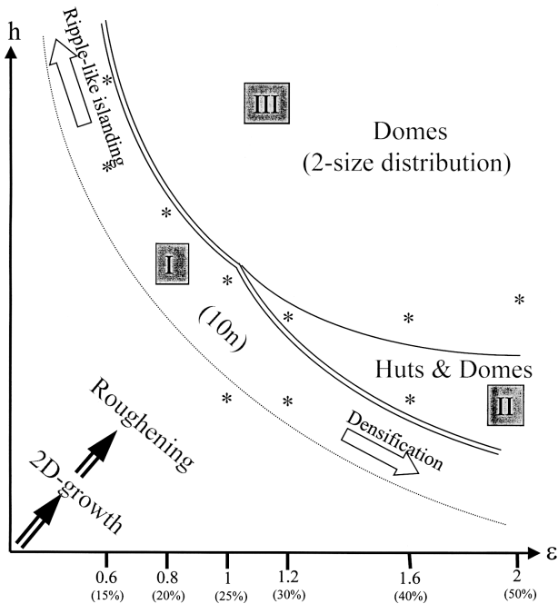
Fig. 2. Schematic ‘kinetic phase diagram’ representing the three main growth regimes (at constant growth temperature \sim 550^\circ\text{C} ). Every regime induces a typical morphology of the as-grown \text{Si}_{1-x}\text{Ge}_x layers. Stars represent some of the experimental data presented in the results.
