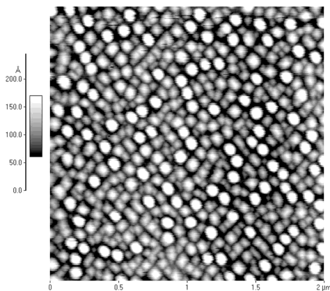
Fig. 7. AFM image of the coexistence of ‘huts’ and ‘domes’ obtained in regime II for \text{Si}_{0.6}\text{Ge}_{0.4} ( h = 5 nm).
