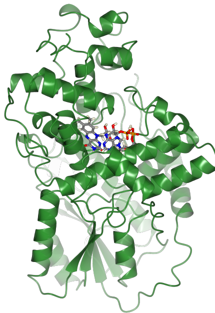
Figure 2: Representation of the arabidopsis thaliana cryptochrome (PDBID: 2J4D) used in the QM/MM simulations. The FAD fragment (ball and stick) constitutes the QM subsystem, while the protein (ribbon) is treated at the MM level. Crystallographic water molecules have been excluded from the plot, but included in the simulations.
