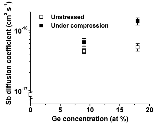
Fig. 4. Variation of the Sb diffusion coefficient measured at 800 °C versus the Ge concentration in unstressed (empty square) and compressively stressed (solid square) \text{Si}_{1-x}\text{Ge}_x layers.
