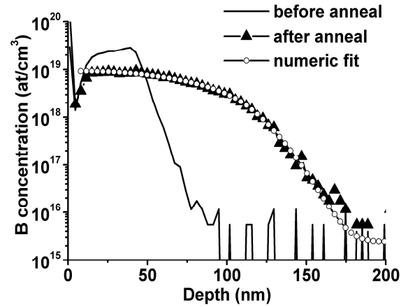
Fig. 2. B concentration profiles measured by SIMS in a relaxed \text{Si}_{1-x}\text{Ge}_x layer ( x = 0.09 ) before (full line) and after (triangles) annealing at 900 \text{ }^\circ\text{C} for 1h, and the simulated profile (open circles) allowing the measurement of the corresponding coefficient of diffusion.
