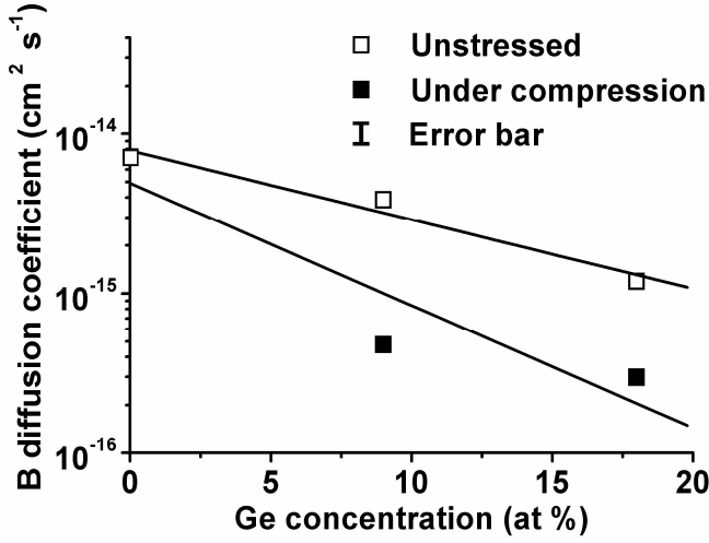
Fig. 3. Variation of the B diffusion coefficient measured at 900 °C versus the Ge concentration in unstressed (empty square) and compressively stressed (solid square) \text{Si}_{1-x}\text{Ge}_x layers.
