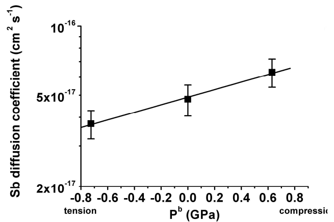
Fig. 6. Variation of the Sb diffusion coefficient at 800 °C with the biaxial pressure ( P^b ) in \text{Si}_{0.91}\text{Ge}_{0.09} .
