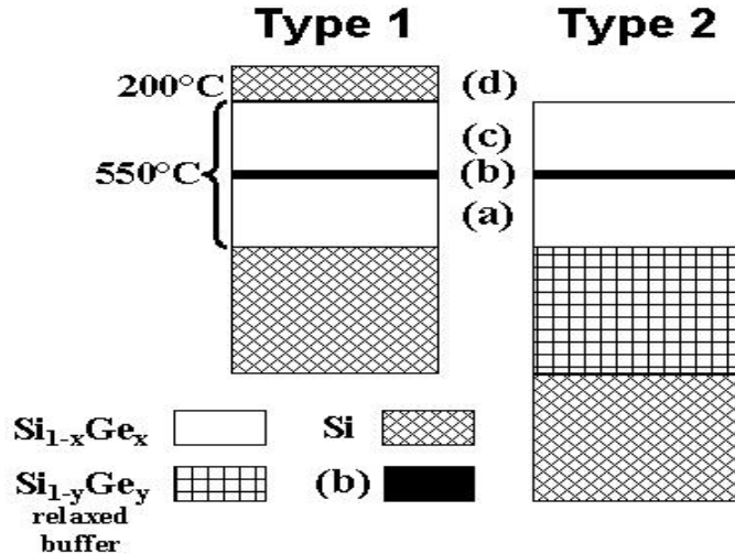
Fig. 1. Schematic presentation of the structures grown by MBE on Si(001). For the type 1 structure, the \text{Si}_{1-x}\text{Ge}_x layer is under biaxial compressive stress. For the type 2 structure, the \text{Si}_{1-x}\text{Ge}_x layer is relaxed if y = x , and under biaxial tensile stress if y > x . The layer (b) located in the middle of the \text{Si}_{1-x}\text{Ge}_x layer is the dopant diffusion source (0.1 monolayer of B or 0.5 monolayer of Sb).
