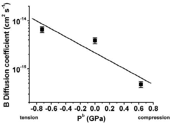
Fig. 5. Variation of the B diffusion coefficient at 900 °C with the biaxial pressure ( P^b ) in \text{Si}_{0.91}\text{Ge}_{0.09} .
