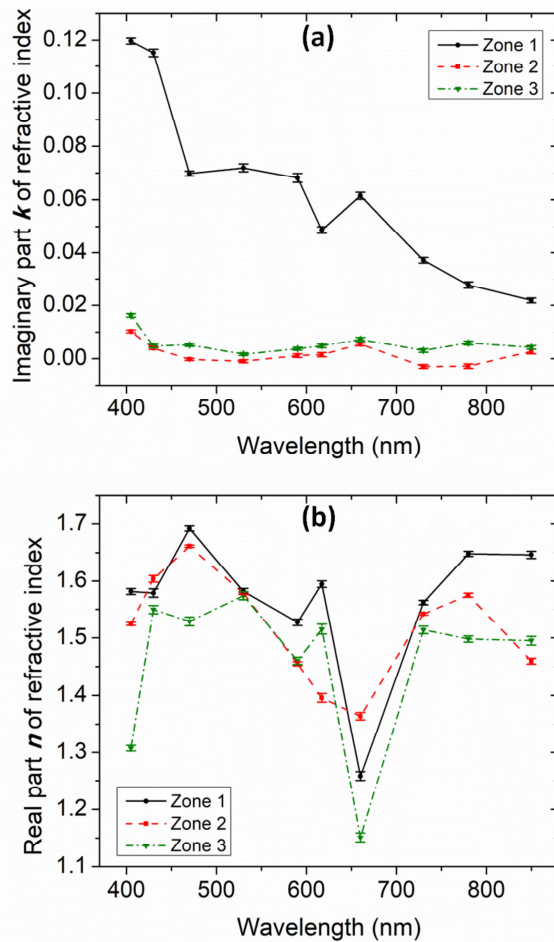
Figure 3: (a) Imaginary part and (b) real part of the refractive index for the different zones of the deposit. Zone 1 is inside a forming crater (representative for growth phase 2). Zone 2 and 3 are outside of the crater (representative for growth phase 1).
