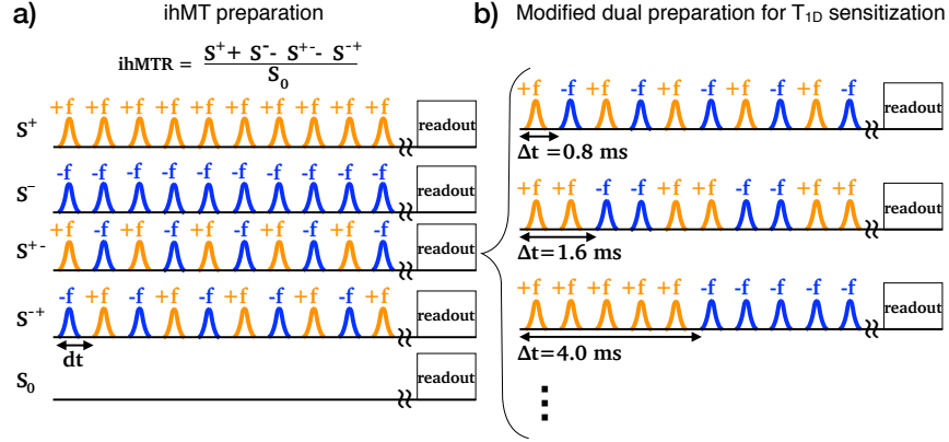
Figure 1: ihMT MRI sequence. a) ihMT preparation including single-offset and dual-symmetric offset saturations. b) Modified ihMT sequence introduced by Varma et al. [20]. In practice, the single-sided off-resonance RF saturation MT image is computed from the average of a MT image obtained with a positive offset ( S^+ ) and one with a negative offset ( S^- ) in order to correct for first order asymmetry effects of g_B arising from the chemical shift of the broad macromolecular lines [36]. For signal-to-noise ratio (SNR) purpose, the dual-sided off-resonance RF saturation is also repeated twice, changing the sign of offset of the pulse ( S^{+-} and S^{-+} ).
