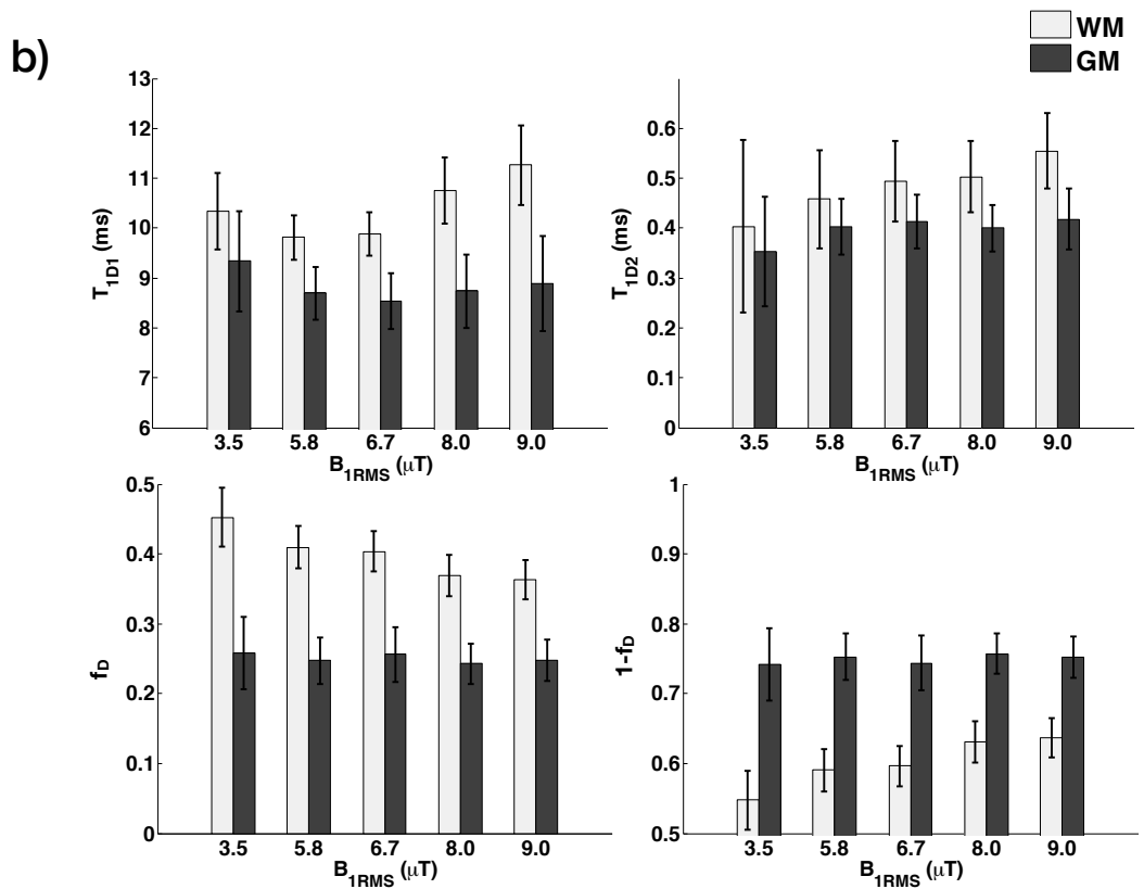
Figure 5: Bi-component T_{1D} model outcomes. a) T_{1D1} , T_{1D2} , f_D , and (1 - f_D) maps of rat spinal cord obtained by using the proposed bi-component T_{1D} ihMT model. b) Bar plots of T_{1D1} , T_{1D2} , f_D and (1 - f_D) values measured in ROIs selected in white (WM) and gray matter (GM) (Fig. 3) for different B_{1RMS} .
