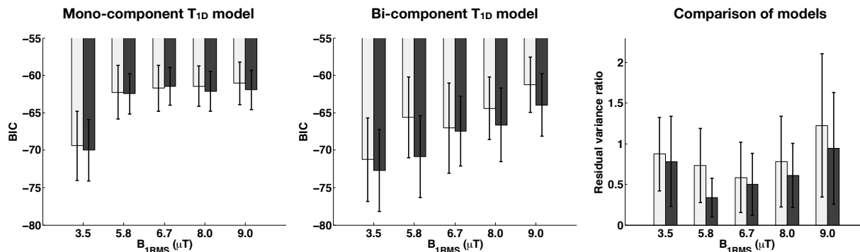
Figure 6: BIC values of each model fit: mono-component (left) and bi-component (middle). Residual variance ratio (bi : mono-component T_{1D} models) for gray and white matter for each B_{1RMS} (right). Values less than one indicate a better performance of the proposed model.
