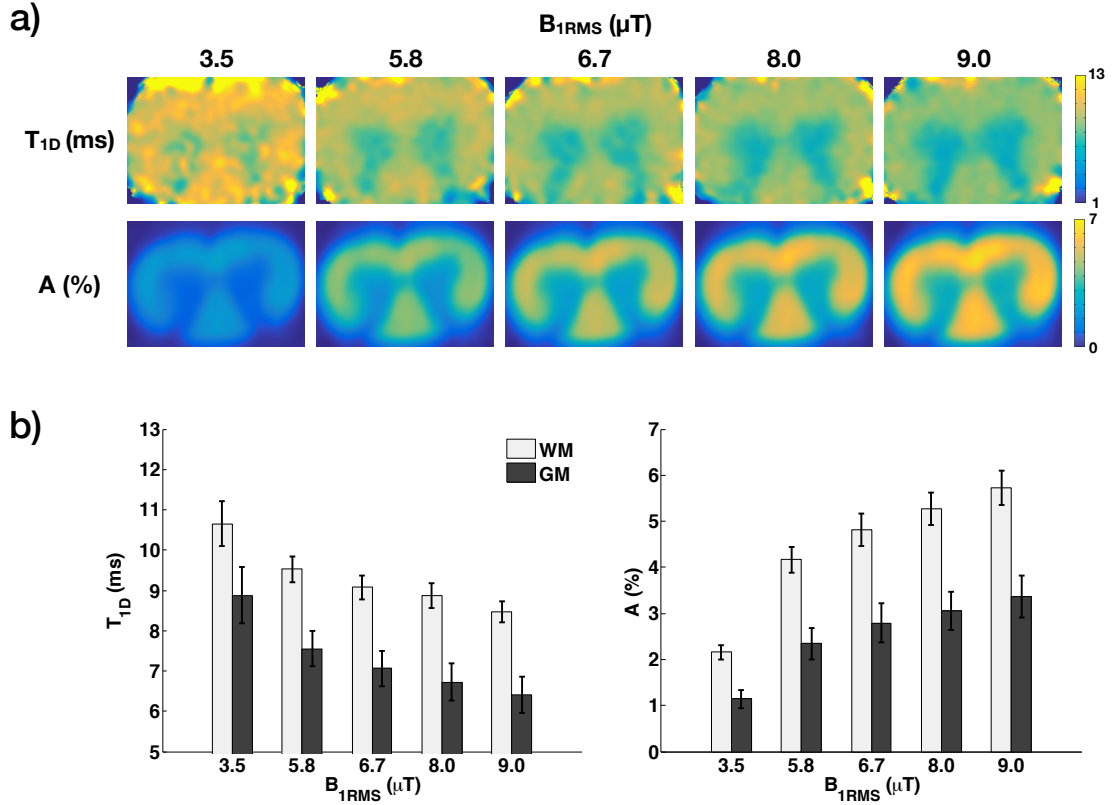
Figure 4: Mono-component T_{1D} model outcomes. a) T_{1D} (upper row) and scaling factor A (lower row) maps of rat spinal cord derived by fitting the analytical solution for the mono-component T_{1D} model [20] to ihMTR( \Delta t ) (Fig. 3). b) Bar plots of T_{1D} (left) and A (right) values measured in ROIs selected in white (WM) and gray matter (GM) (Fig. 3) for different B_{1RMS} .
