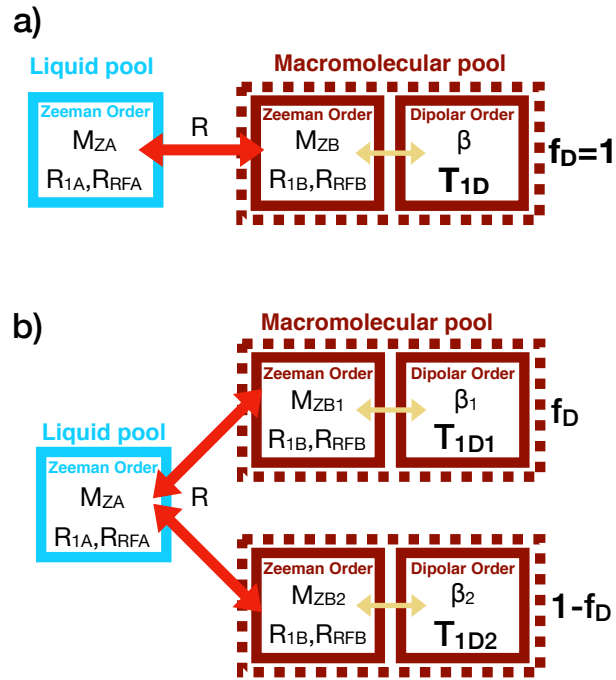
Figure 2: A) Mono-component T_{1D} ihMT model presented in [20]. B) Proposed bi-component T_{1D} ihMT model.
