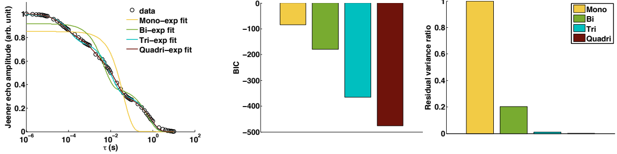
Figure 7: (left) Jeener-Broekaert echo decays in a synthetic membrane (POPC: 40%; cholesterol 40%; cerebrosides 20% (molar ratio)) and fitted with multi-exponential models. (middle) BIC values of each exponential model fit. (right) Residual variance ratio between each exponential model and the mono-exponential model.
