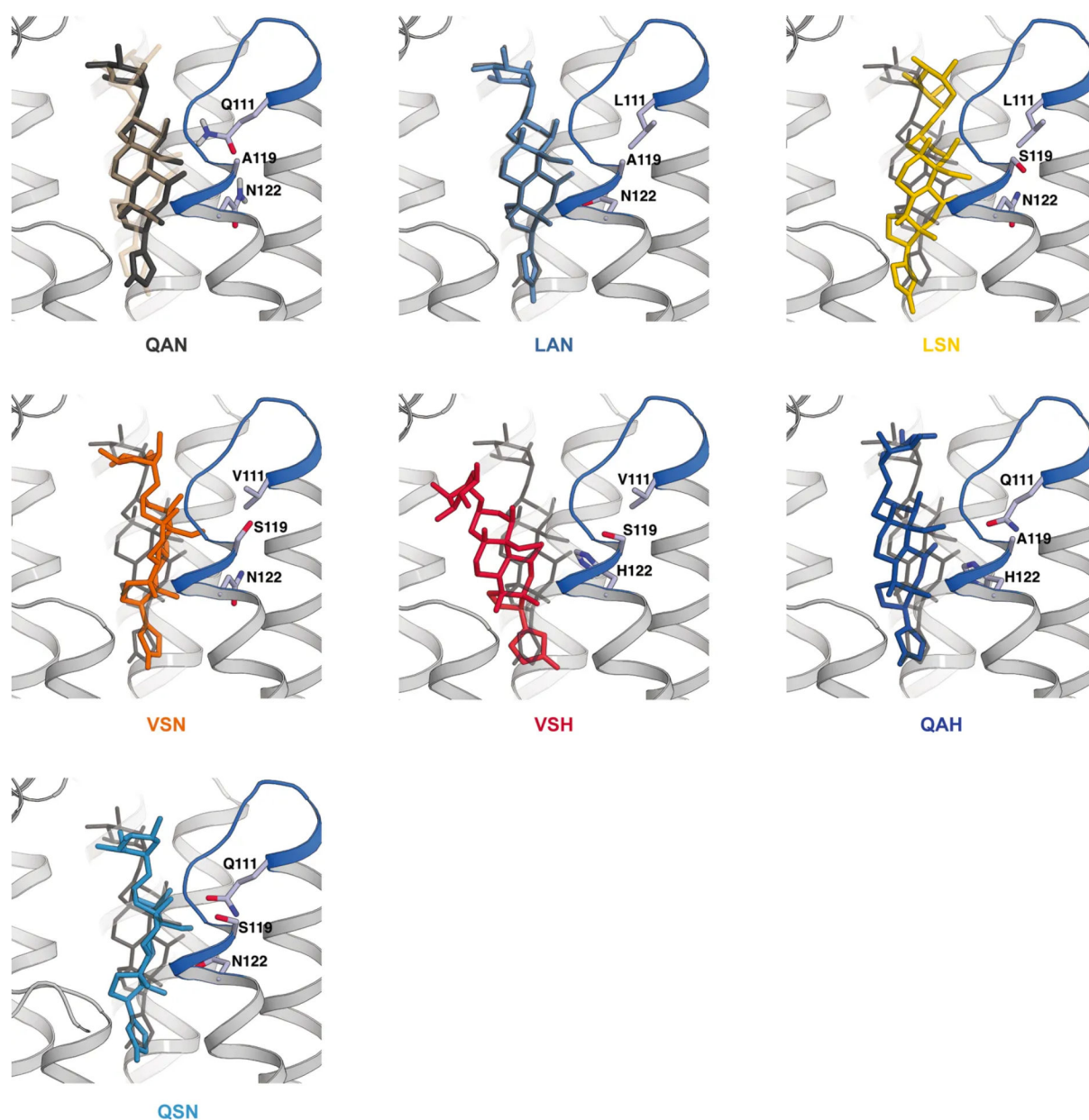
Extended Data Fig. 9. Molecular docking simulations show stepwise reductions in ouabain binding to \text{Na}^+/\text{K}^+ -ATPases with monarch lineage substitutions in \text{ATP}\alpha .
