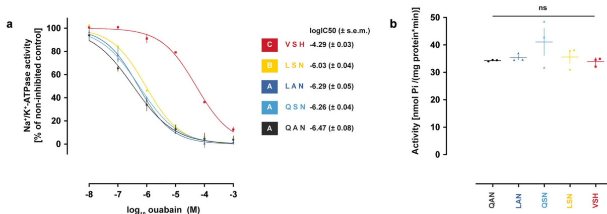
Extended Data Fig. 8. The Atpa genotypes found along the monarch lineage sequentially increase TSI to ouabain without affecting baseline levels of sodium pump activity.
