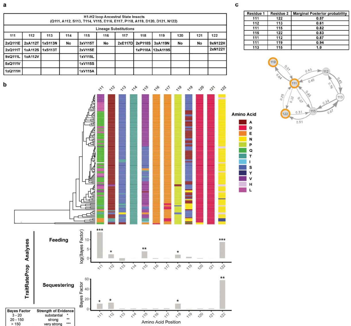
Extended Data Fig. 1. Substitutions at ATP \alpha amino acid residues 111, 119 and 122 are directly or indirectly associated with insect specialization on plants that produce cardiac glycosides.
