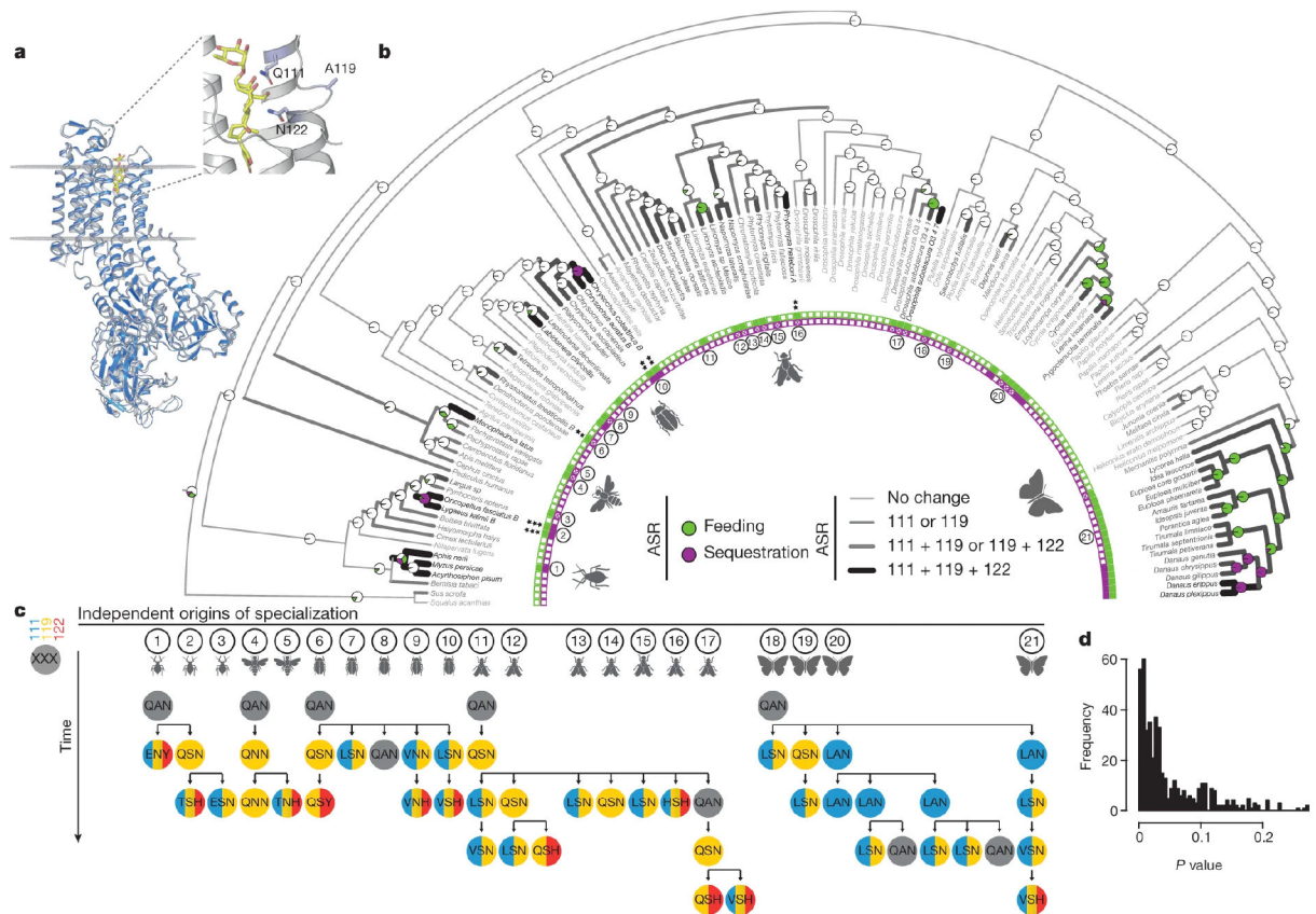
Fig. 1. Mutational paths in ATPα associated with insect specialization on cardiac glycoside-producing plants are constrained.
