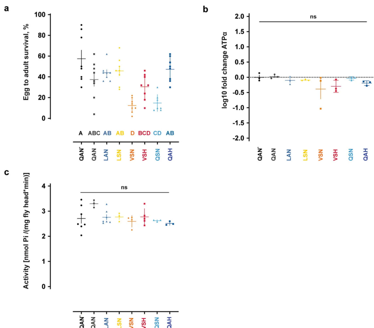
Extended Data Fig. 3. Point mutations have some effect on adult emergence, but do not lead to major changes in baseline Atpα expression or \text{Na}^+/\text{K}^+ -ATPase activity.
