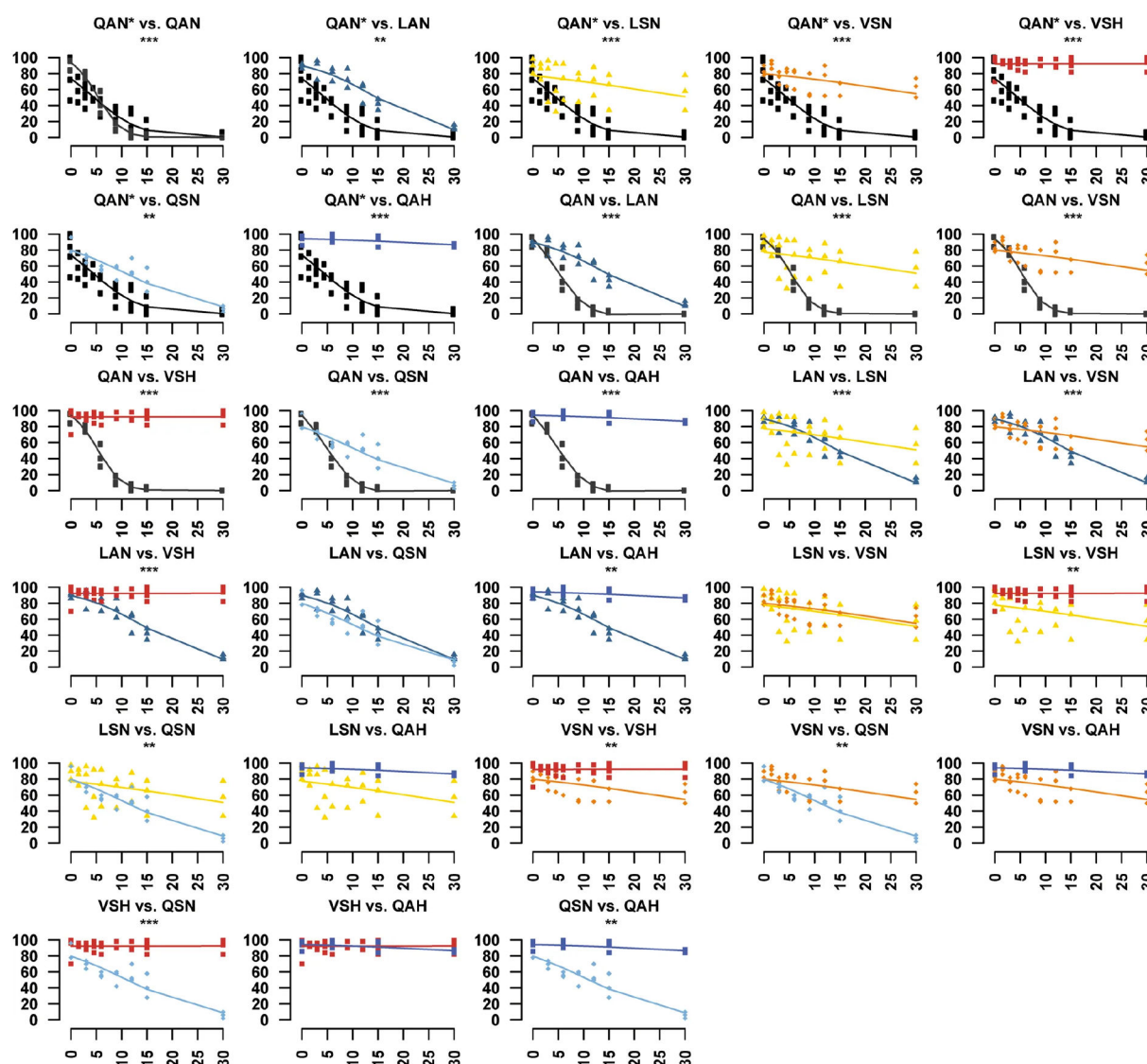
Extended Data Fig. 4. Drosophila flies with edited genomes show increased larval–adult survival when fed cardiac glycosides.
