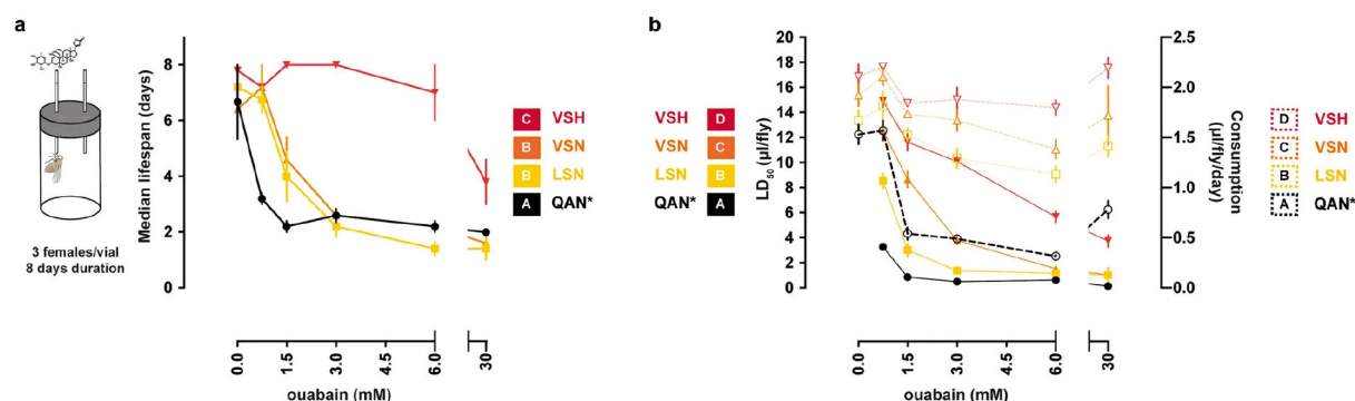
Extended Data Fig. 6. The mutational path of ATP \alpha in the monarch butterfly lineage increases dietary tolerance to ouabain in vivo in engineered Drosophila without affecting feeding rate.
