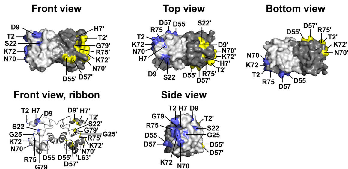
FIGURE 1 | Wildtype BANF1 residues affected by novel ExAC missense variants. Crystal structure (Umland et al., 2000) of the BANF1 dimer showing wildtype residues affected by novel ExAC variants (RCSB Protein Data Bank ID: 1CI4). 'Top' and 'Bottom' views were obtained by rotating the 'Front view' 90° along its long axis out of, and into, the page respectively. 'Side view' shows the DNA-binding surface of BAF and was obtained by rotating the Front view 90° to the right. Wildtype residues affected by ExAC variants are colored blue in the pale-gray subunit, and yellow in the dark-gray subunit. Plain and 'prime' numbers indicate affected residues in the pale-gray and dark-gray subunits, respectively. Ribbon depiction of the 'Front view' reveals residues involved in the dimer interface, and a buried \alpha -helical residue that we predict is disrupted by variant p.L63P.
