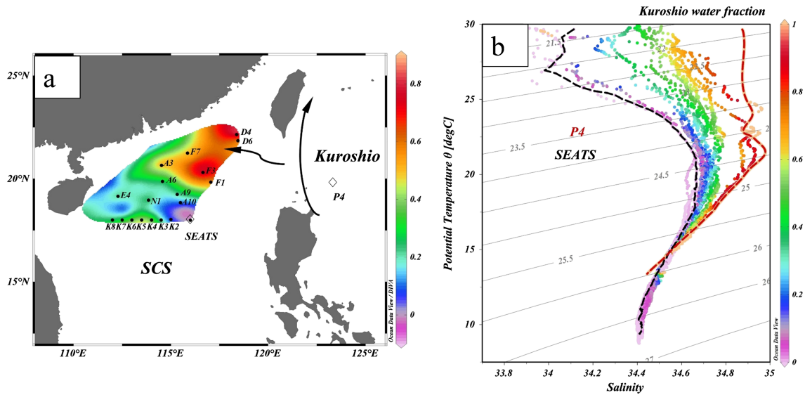
Figure 1. (a) The spatial pattern of the KI index. The color bar represents the value of R_{kave-100} . Black solid dots represent the sampling stations. The two open diamonds are the two end member stations (SEATS for the SCS and P4 for the Kuroshio) chosen for the isopycnal mixing model. (b) \theta -S diagram of the upper 400 m for all the investigated stations. The red dashed curve denotes typical Kuroshio water, and the black dashed curve denotes typical SCS water. KI = Kuroshio intrusion; SCS = South China Sea.
