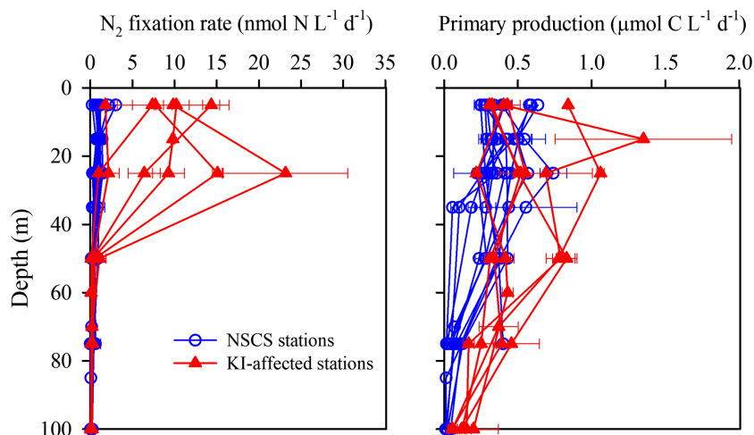
Figure 3. The vertical profiles of N_2 fixation rate ( \text{nmol N}\cdot\text{L}^{-1}\cdot\text{d}^{-1} ) and primary production ( \mu\text{mol C}\cdot\text{L}^{-1}\cdot\text{d}^{-1} ) at incubation stations. NSCS = northern South China Sea; KI = Kuroshio intrusion.
