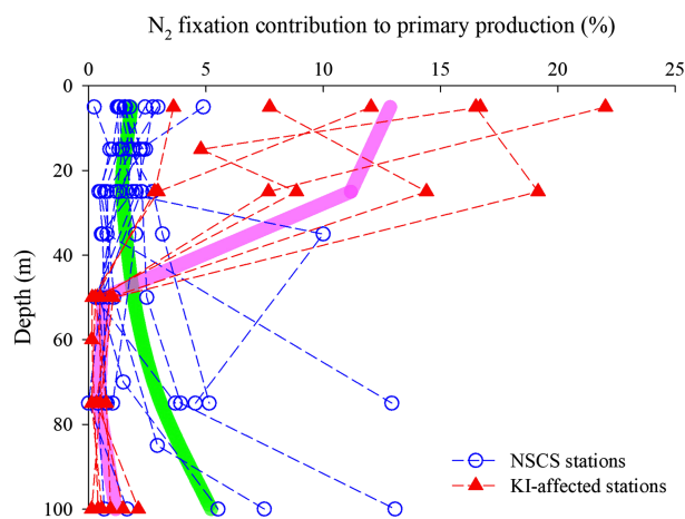
Figure 5. The depth distribution of N_2 fixation contribution to the N demand of primary production based on Redfield ratio of 6.6. The green and pink lines represent the average contribution of N_2 fixation to primary production in the NSCS region and KI-affected region, respectively. NSCS = northern South China Sea; KI = Kuroshio intrusion.
