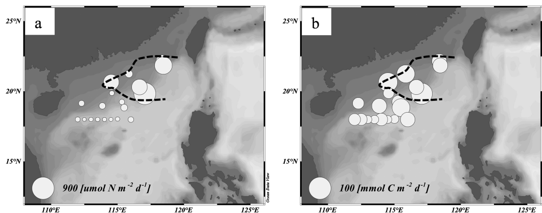
Figure 4. Spatial distributions of (a) the depth-integrated N_2 fixation rate ( \mu\text{mol N}\cdot\text{m}^{-2}\cdot\text{day}^{-1} ) and (b) depth-integrated primary production ( \text{mmol C}\cdot\text{m}^{-2}\cdot\text{day}^{-1} ). The dashed curves represent the isopleth of Kuroshio intrusion index of 0.5.
