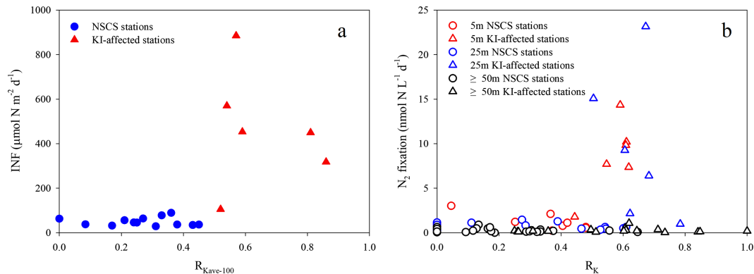
Figure 7. (a) The depth-integrated (upper 100 m) N 2 fixation rate (INF, \mu\text{mol N}\cdot\text{m}^{-2}\cdot\text{day}^{-1} ) against the average Kuroshio fraction in the upper 100 m; (b) N 2 fixation rate ( \text{nmol N}\cdot\text{L}^{-1}\cdot\text{day}^{-1} ) against the Kuroshio fraction at each depth (5, 25, and 50 m). NSCS = northern South China Sea; KI = Kuroshio intrusion.
