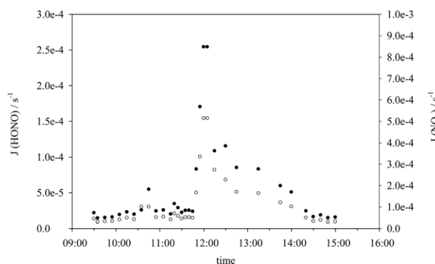
Fig. 2 The photolysis rate constants of HONO (B) and NO 2 (C) in the period between 9:30 a.m. and 3 p.m. on December 3 rd , in the lab room in Guangzhou.
