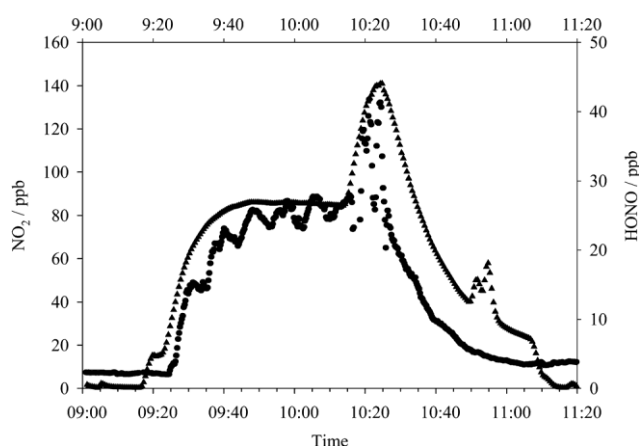
Fig. 3 The mixing ratios of (□) HONO and (○) NO 2 during a cooking event at December 07 2018 in the lab room on the campus at JNU, Guangzhou, China. The combustion started with \frac{1}{2} flame at 9:17. At 10:20, the knob of the gas appliance was turned to the maximum. The sharp increase of both NO 2 and HONO mixing ratios at 10 : 20 correspond to the increased combustion regime (maximum gas flame) of the gas appliance.
