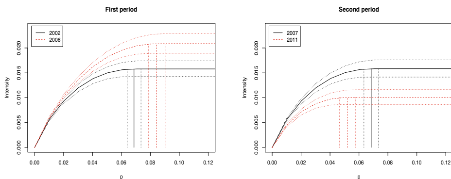
Fig. 4 The three I's of child poverty in Germany. (90% credible intervals are represented by dotted lines. In black solid line is represented the TIP curve at the beginning of each sub-period. The red dashed line corresponds to the TIP curve of the end of each subperiod.)
