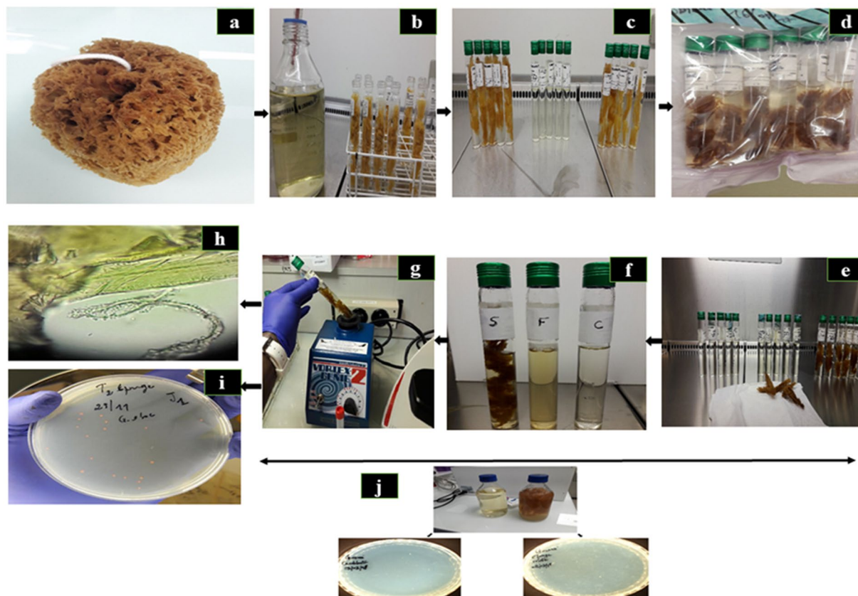
Figure 3. The main steps of experimental procedure: (a) Dead Spongia Sp. skeleton were washed and dried. (b) Sponges were cut into small pieces of uniform size and 0.5 g were introduced in glass tubes before adding 15 mL Caulobacter liquid medium (CLM). (c) The three-liquid media before autoclaving: ten glass tubes containing 0.5 g small fractions of sponges immersed in 15 mL CLM (medium B), and five glass tubes containing 15 mL. (d) Marine sponges immersed in the CLM after autoclaving at 121 °C/15 min e. The three media after autoclaving: at left to right: control medium, medium B (prepared as described for medium A except that the 0.5 g small pieces of sponge tissue have been removed after autoclaving and filtered and medium A (a liquid–solid biphasic system). The final volume of culture at 15 mL was then completed after an adjustment with each corresponding liquid medium after autoclaving in order to compensate the liquid evaporated. (f) The characteristics of the three liquid media prepared to be inoculated. (S) for sponge medium, (F) for filtrate and (C) for CLM. (g) Procedure of vortex. Each tube was vortexed for 1 \times 10 s and broth was removed to perform serial dilutions followed by subculture onto agar solidified medium on 100-mm Petri dishes. Vortex procedure was repeated ( 4 \times 10 s) until a constant enumeration was obtained. Bacterial growth was monitored by microscopy (using kova slides) (h) and CFUs enumeration (i) in parallel. (j) Culture on solid media. For control medium and sponge filtrate medium, 15 g/L of agar were added to prepare corresponding solid media: sponge filtrate (F) solid medium, and (C) Caulobacter solid medium.
