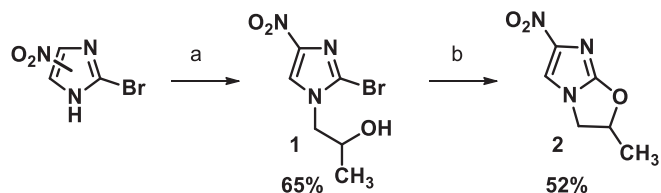
Scheme 1. Synthesis of 6-nitroimidazooxazole 2: a) propylene oxide (1.5 equiv.), DIPEA (5 equiv.), 110 °C, MW, 1.5 h. b) NaH (2 equiv.), DMF, N_2 , 0 °C, 65 min.
