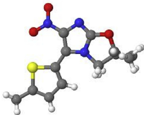
Fig. 4. X-ray structure of compound 5h .
