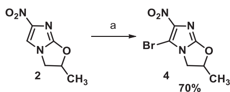
Scheme 2. Synthesis of 5-bromo-2-methyl-6-nitro-2,3-dihydroimidazo[2,1-b]oxazole 4 : a) NBS (1 equiv.), CH 3 CN, rt, 1 h.
