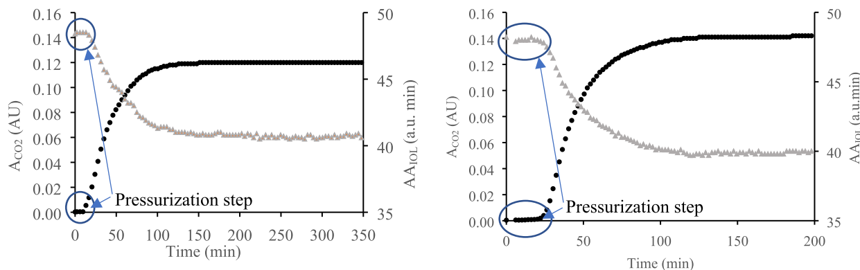
Fig. 5. Evolution of CO 2 peak absorbance at 4950 cm -1 ( A_{\text{CO}_2} ) ( \bullet ) and integrated area of IOL peak in the range of 5500–6000 cm -1 ( AA_{\text{IOL}} ) ( \blacktriangle ) with contact time at 308 K and 8 MPa (left) and 25 MPa (right).
