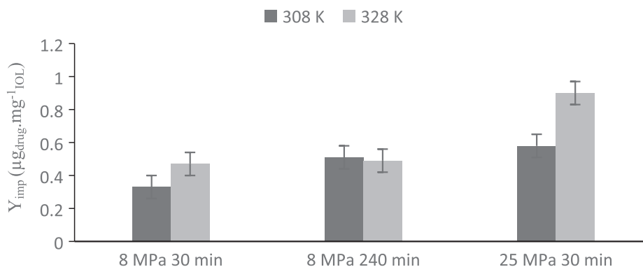
Fig. 9. Influence of temperature on IOL impregnation yield at different experimental conditions.
