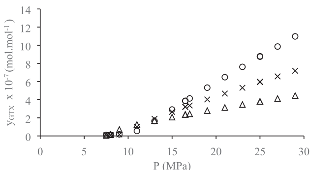
Fig. 4. Gatifloxacin solubility in supercritical CO 2 ( y_{\text{GTX}} ) at ( \Delta ) 308 K, ( \times ) 318 K and ( \circ ) 328 K calculated using data from (Shi et al., 2017).
