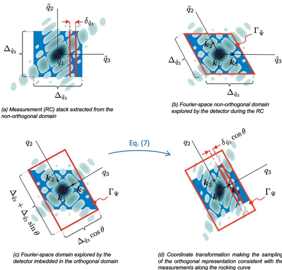
Figure 4 Non-orthogonal and orthogonal representations of the diffracted far field in the Bragg geometry. (a) The 3D stack of intensity measurements obtained during the RC, as stored in a 3D array, (b) is produced by the regular sampling of the far field \Psi performed within the non-orthogonal measurement domain imposed by the detector geometry and delimited by the shaded area \Gamma_{\tilde{\Psi}} . (c) In an orthogonal basis, the far field \Psi computed in a domain \Gamma_{\Psi} can be defined to contain the non-orthogonal domain \Gamma_{\tilde{\Psi}} . In addition, after the coordinate transformation given in (7), \Psi provides a computed representation of the far field whose sampling is totally consistent with the data (RC) stack (d). Because the non-orthogonal measurement domain \Gamma_{\tilde{\Psi}} shown in (d) is smaller than \Gamma_{\Psi} , the computed representation of \Psi in \Gamma_{\Psi} is not totally constrained by the intensity measurements shown in (b). For the sake of the demonstration, a cubic sample has been numerically designed, with its Bragg vector pointing towards one of its edges. Note the agreement between (a) and (d).
