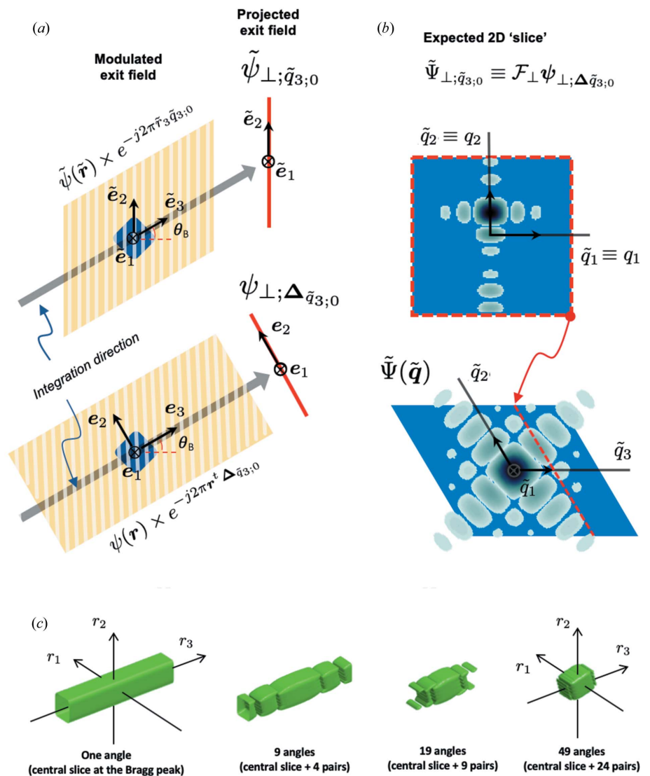
Figure 5 Illustration of the projection/back-projection strategy. (a) The integrated exit field in the non-orthogonal or in the orthogonal real-space representation allows us to derive (b) a ‘slice’ \tilde{\Psi}_{\perp; \tilde{q}_{3;0}} extracted from \tilde{\Psi}(\tilde{\mathbf{q}}) at \tilde{q}_3 = \tilde{q}_{3;0} . (c) Conversely, the summation of a series of back-projections allows us to retrieve the object from its evenly sampled ‘slices’; here, the retrieved sample is converging toward the cubic real-valued particle shown in Fig. 3.
